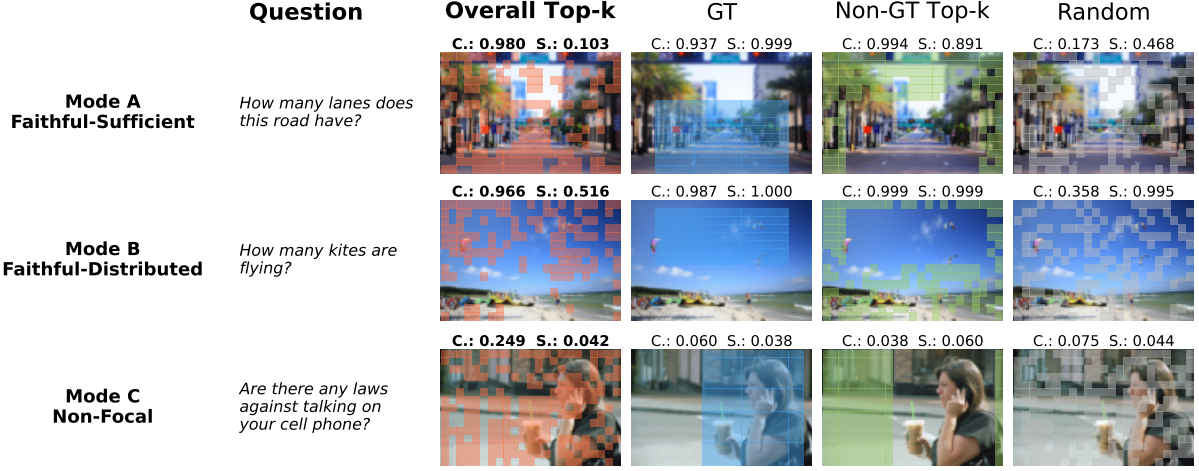
Figure 3: Representative samples for the three processing modes. Each row visualizes the four perturbation strategies on a representative case and reports the per-strategy normalized comprehensiveness (C.) and sufficiency gap (S.), illustrating why the top- k tokens are sufficient in Mode A, only necessary in Mode B, and almost inert in Mode C.
