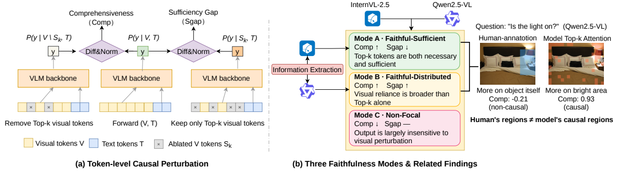
Figure 1: Overview of the proposed evaluation framework and main findings. (Left) Visual attention faithfulness is evaluated using comprehensiveness and the sufficiency gap under token-level perturbations, by respectively removing or retaining top- k attention-ranked visual tokens. (Right) Three faithfulness modes of visual attention of the VLM backbone. Different VLM architectures may handle the same task in different modes, for example, the IE task. Furthermore, what humans perceive as causal regions is not always the focus of the model’s attention.
