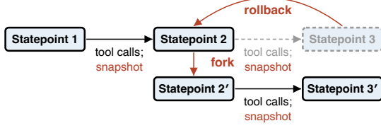
Figure 3. State management primitives for agent statepoints
