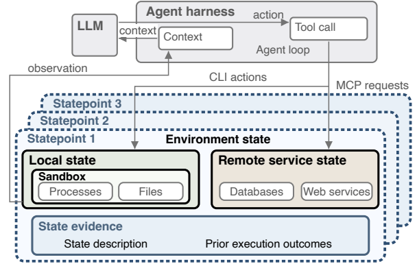
Figure 2. Overview of agent statepoints
