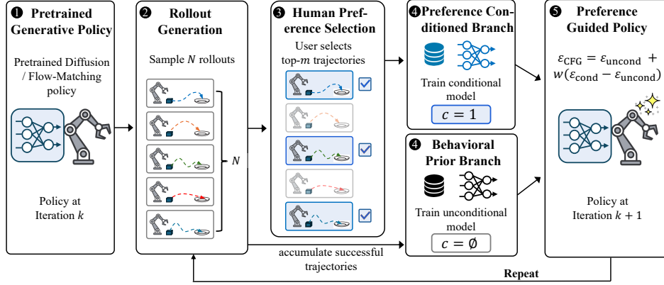
Figure 2: Overview of PrefPI. Each iteration trains two branches, one conditioned on the top- m rollouts and the other on all successful rollouts, and CFG combines the two branches to produce the next policy.
