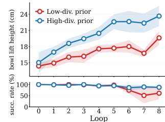
Figure 8: PrefPI benefits from a high-diversity prior.
