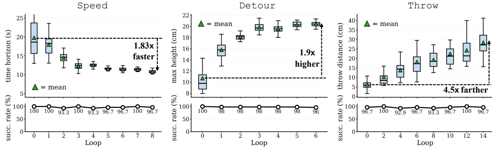
Figure 5: Real-world steering on three different preferences. PrefPI improves the preference metric by 1.83\times (speed), 1.9\times (detour), and 4.5\times (throw), while success rates remain above 90%.
