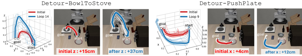
Figure 4: Trajectories before and after training are highly disjoint, indicating that the blue trajectories lie beyond the initial policy’s effective support.
