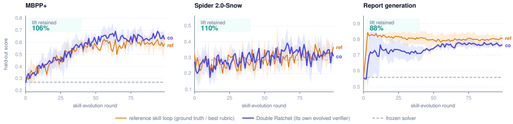
Figure 4: Held-out learning curves (mean \pm std, three seeds): the reference skill loop on ground truth or the best available rubric, against Double Ratchet on its own evolved verifier. Callout: co-evolution’s lift retention as a fraction of the reference loop’s. Held-out evaluation never passes through the evolved verifier.
