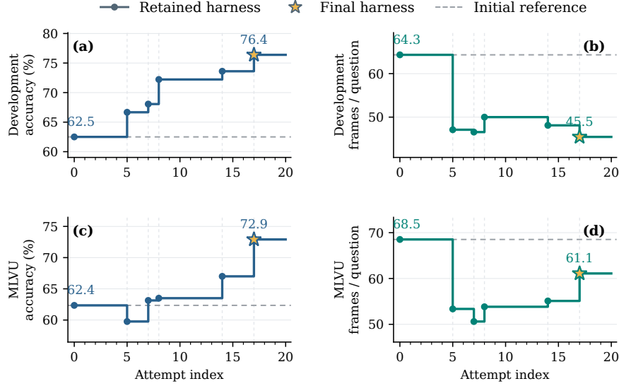
Figure 3: Evolution over 20 revision attempts. Accuracy and mean frames per question on (a,b) the development set and (c,d) MLVU. Curves track the retained harness. Vertical guides mark accepted revisions, and flat intervals indicate an unchanged incumbent.
