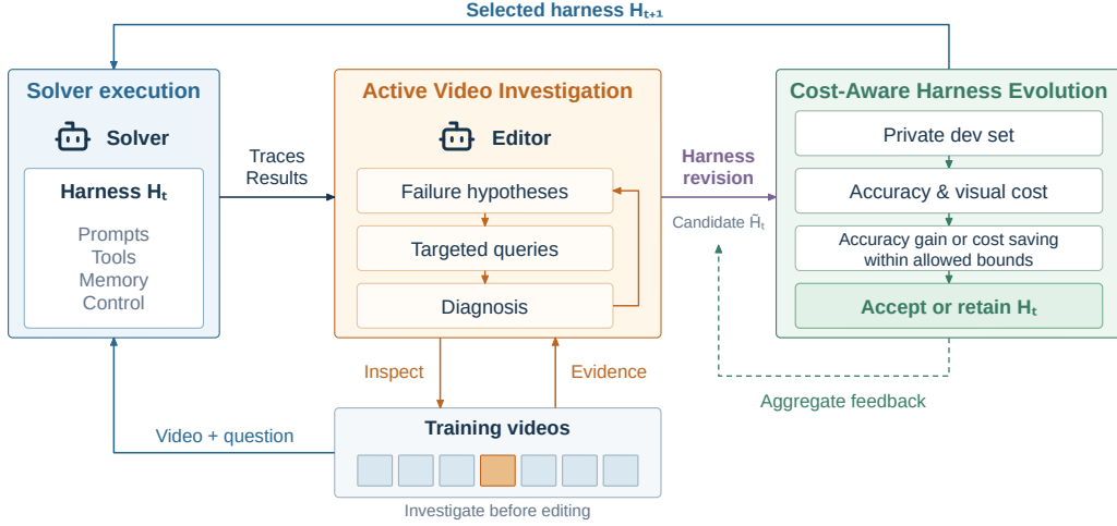
Figure 2: Overview of Video-RSI. The Solver and Editor share a frozen language model. Active video investigation revisits training videos to diagnose failures and guide harness revisions. Cost-aware harness evolution selects candidates using accuracy and visual cost on a private development set, carrying accepted revisions into subsequent iterations.
