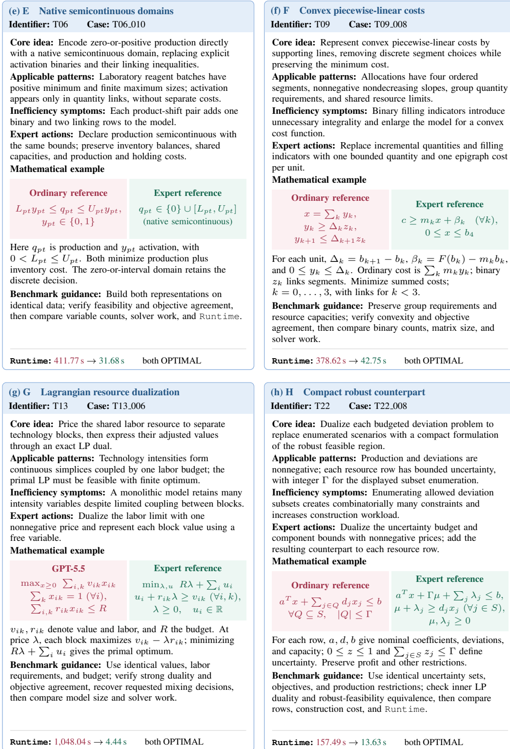
Figure 13: OptTips cards for families E–H. The same seven-component schema continues with four further examples. Panel (g) retains the GPT-5.5–expert comparison from Figure 1; other panels use ordinary and expert references. Times report solver Runtime under the execution protocol in Appendix D; panel (h) lacks historical input-hash verification.
