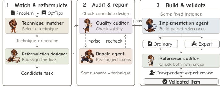
Figure 4: OptDachshund workflow: from source problems to validated tasks with ordinary and expert references.
