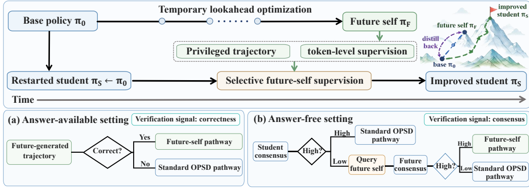
Figure 1: Overview of B-OPSD. We first train the base policy \pi_0 forward to obtain a future self \pi_F , then restart the student from \pi_0 and distill from \pi_F when future supervision is reliable. The future self supplies both privileged trajectories and token-level targets. In the answer-available setting, reliability is determined by correctness; in the answer-free setting, it is determined by student and future consensus.
