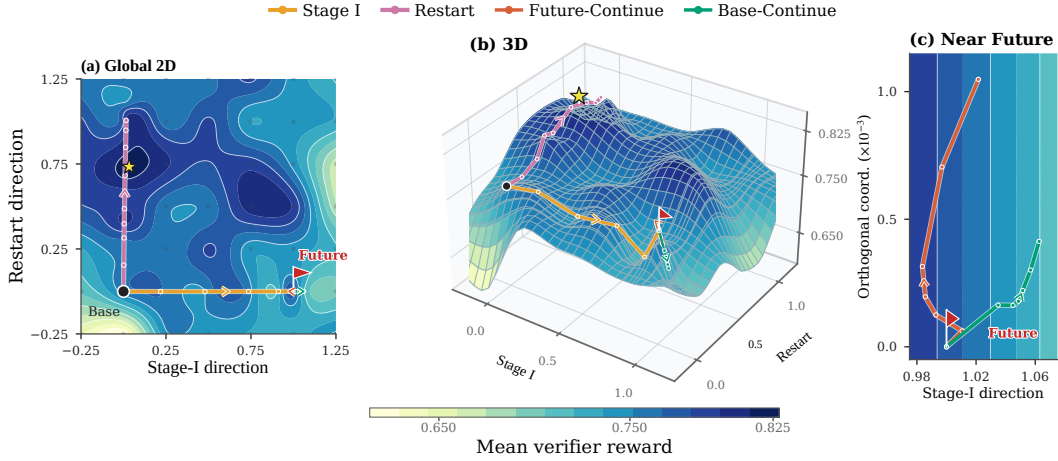
Figure 2: Optimization trajectories under restart and continuation. (A) Two-dimensional verifier-reward landscape and optimization trajectories in a shared parameter plane. (B) Corresponding three-dimensional view. (C) Magnified view around \pi_F , showing the two continuation trajectories. Darker colors indicate higher reward on the held-out problems. The red flag marks \pi_F , small dots denote evaluated grid models, circular path markers denote evaluated training checkpoints, and the star marks the maximum of the interpolated surface.
