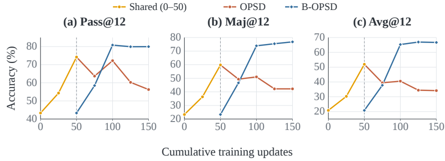
Figure 3: Comparison of AIME25 performance at matched cumulative update budgets for Qwen3-8B. The gray line in each panel marks the end of future-policy construction. The B-OPSD curve begins there with the student restored to \pi_0 , while OPSD continues from \pi_{50} .
