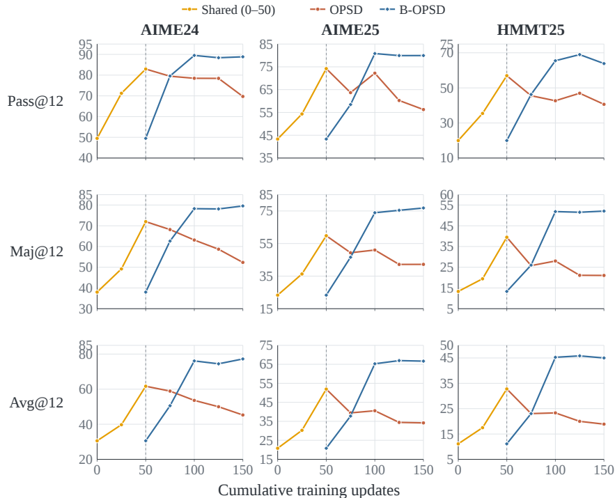
Figure 4: Matched-budget training dynamics across benchmarks and metrics. Columns show AIME24, AIME25, and HMMT25; rows show PASS@12, MAJ@12, and AVG@12. The gray dashed line marks the end of the 50 lookahead updates. The curves are compared at shared cumulative budgets of 50, 75, 100, 125, and 150 updates.
