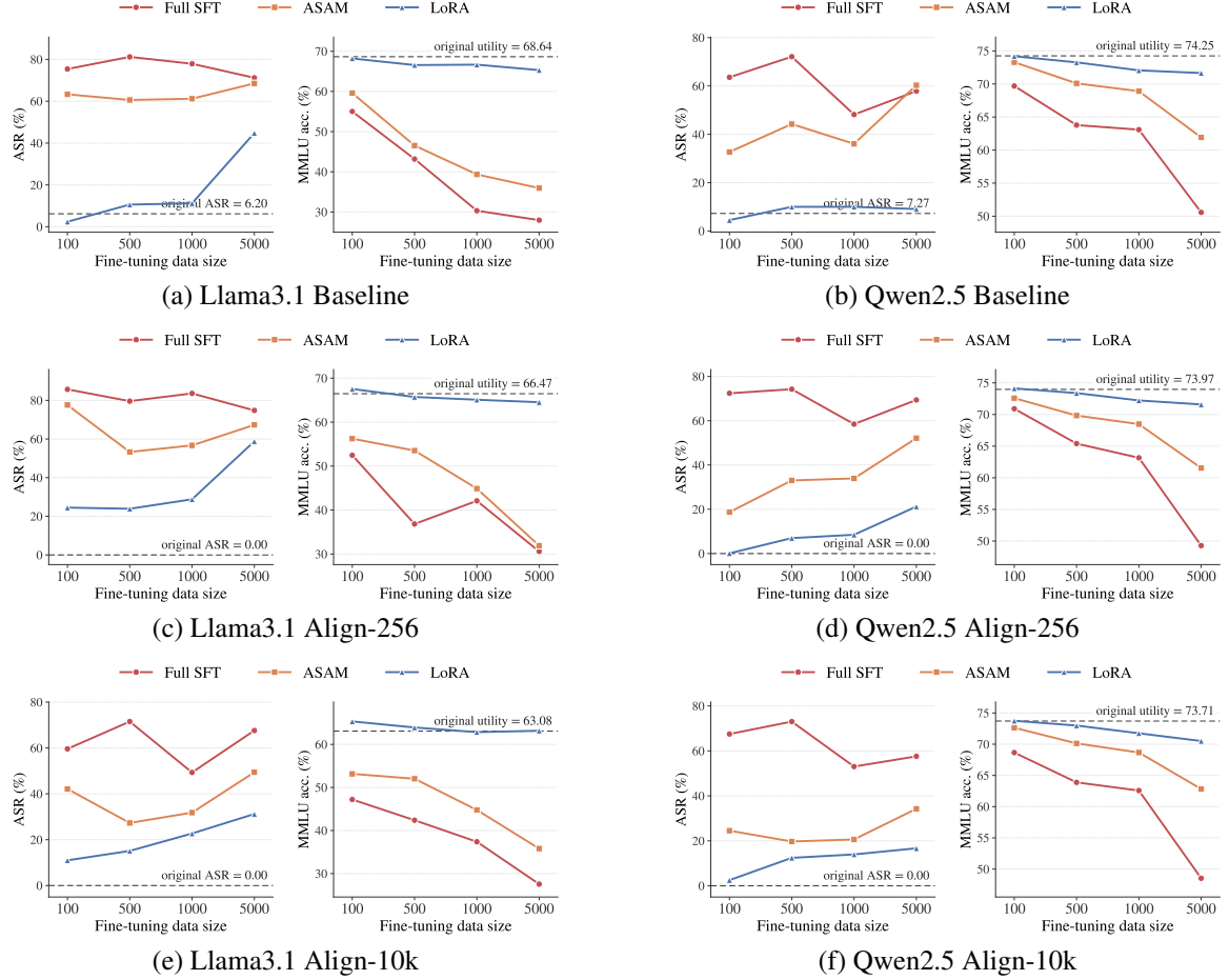
Figure 7: ASR and utility (MMLU) scaling across model families and alignment settings.
