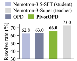
Figure 4 | SWE-Bench Verified results. PIVOTOPD improves more than OPD.
