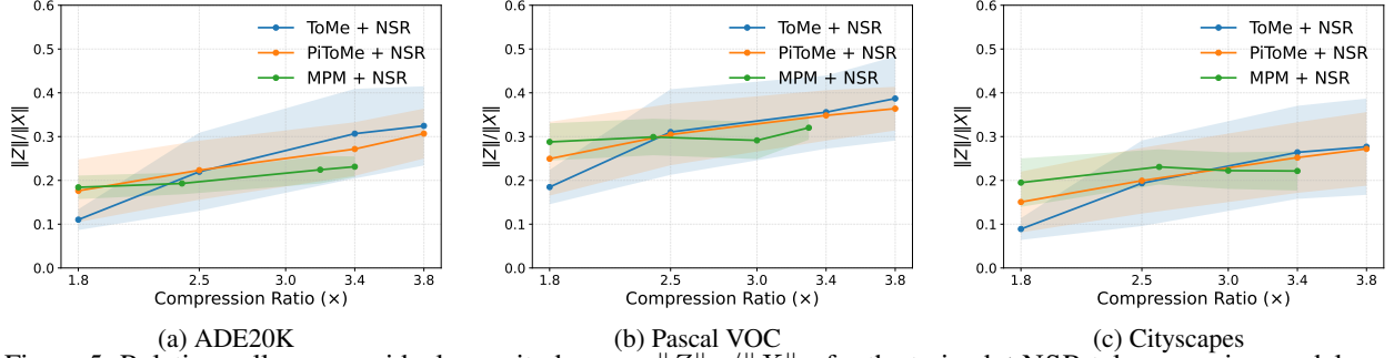
Figure 5: Relative null-space residual magnitude \rho_Z = \|Z\|_F / \|X\|_F for the trained +NSR token-merging models on (a) ADE20K, (b) Pascal VOC, and (c) Cityscapes. For each compression setting, the solid line reports the mean across merging blocks in which NSR is constructed, and the shaded region shows the corresponding mean \pm one standard deviation.
