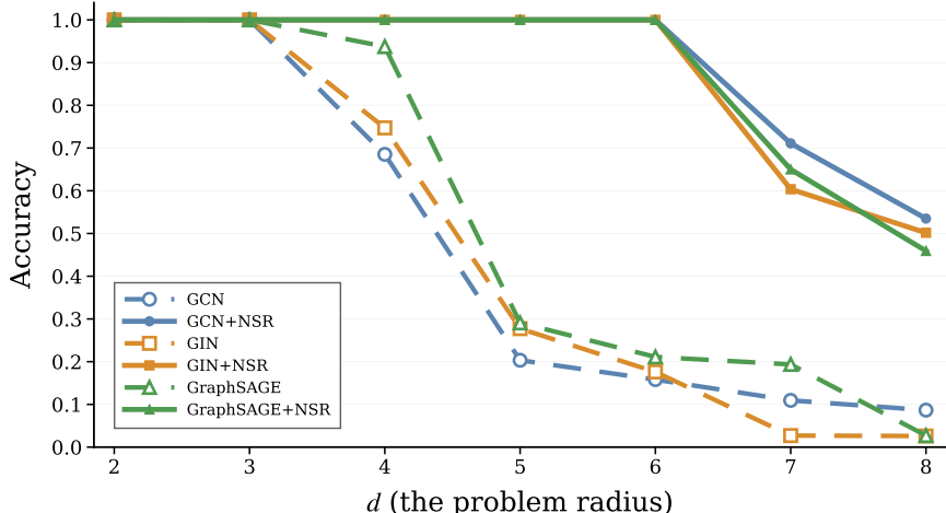
Figure 3: Training accuracy on Tree-NeighborsMatch across tree depths. Dashed and solid curves denote the original GCN, GIN, and GraphSAGE models and their NSR variants, respectively. Each point is the highest training accuracy attained in the corresponding run.
