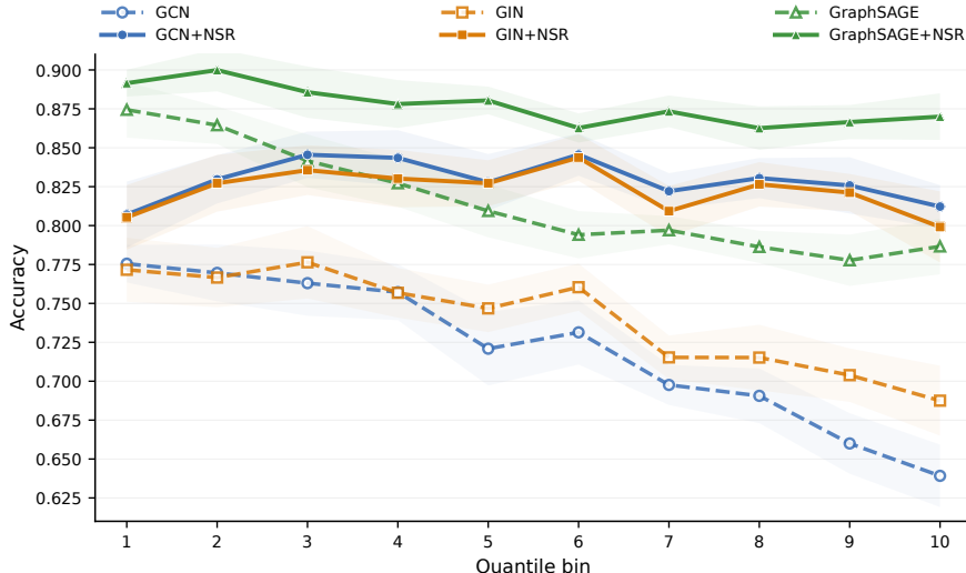
Figure 4: Within each official split, test nodes are divided into ten approximately equal-frequency bins, with the horizontal axis ordering the bins from low to high scores. Lines show the mean accuracy of the corresponding bin across the ten official splits, and shaded bands of the same color indicate the mean \pm one sample standard deviation.
