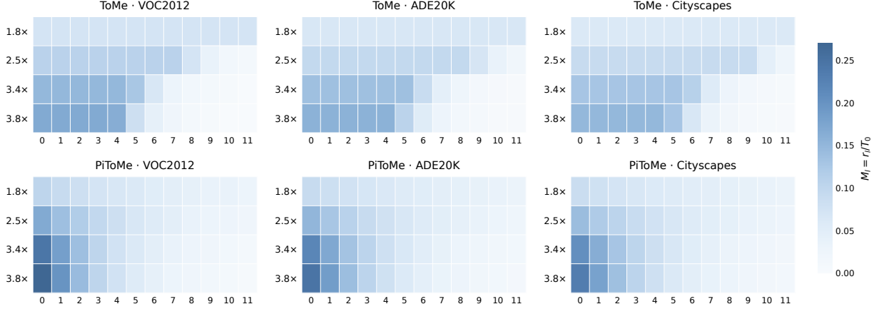
Figure 7: Layer-wise token-merging distributions of ToMe and PiToMe on VOC2012, ADE20K, and Cityscapes. The top and bottom rows correspond to ToMe and PiToMe, respectively, while the three columns correspond to VOC2012, ADE20K, and Cityscapes from left to right. The horizontal axis indicates the Transformer block index, and the vertical axis indicates the target computation-reduction factor. Color represents the normalized number of merged tokens, M_l = r_l / T_0 . All subplots share the same color scale, with darker colors indicating a larger fraction of the initial patch tokens merged at the corresponding block.
