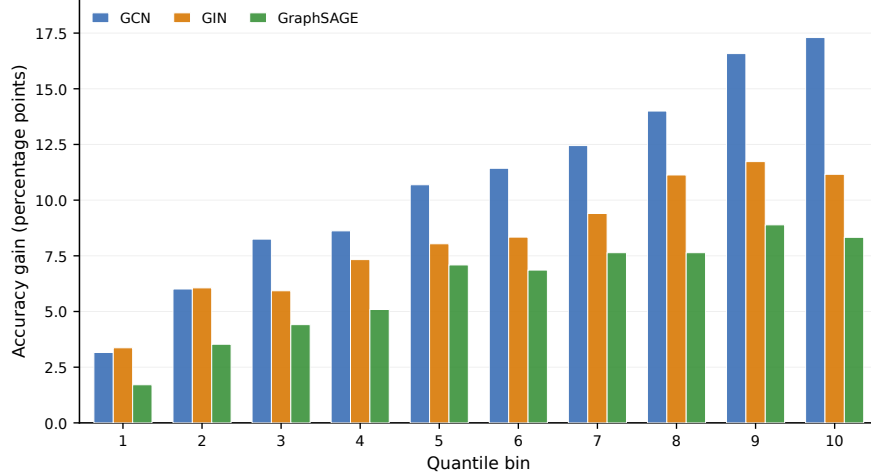
Figure 6: Mean accuracy gain from NSR across diagnostic-score bins on Roman-empire. Bins are the same as those in Figure 4. Within each official split, the gain is computed as the accuracy of the NSR-augmented model minus that of the Original model. The figure reports the mean over the ten official splits.
