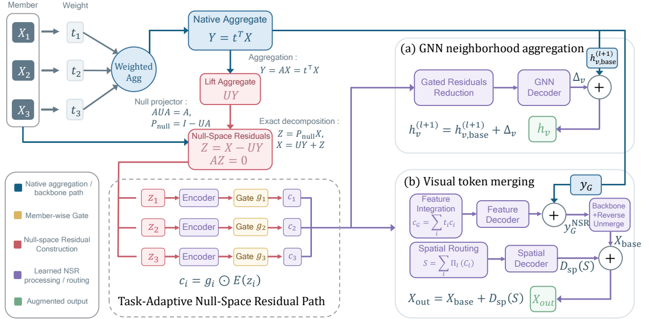
Figure 2: Overview of NSR. Null-space residuals are extracted from pre-mapping representations based on the current linear operator and transformed into usable complementary information through a learnable branch under task supervision. The original mapping branch retains its computation rule.
