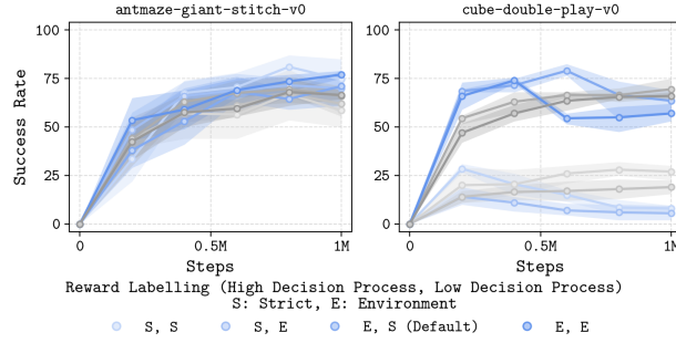
Figure 12: Strict versus environment dataset reward labelling ablation for QSO (blue) and ASO (grey).
