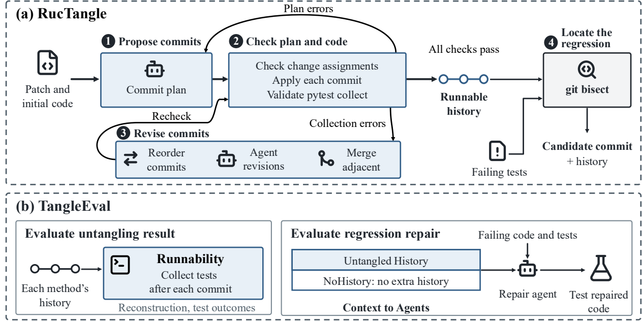
Figure 2. RUCtANGLE and its use in TANGLEVAL. (a) RUCtANGLE checks and revises agent-proposed ordered commits to keep each version runnable, then uses git bisect to identify a candidate commit for regression repair. (b) TANGLEVAL evaluates untangling results and agents’ performance in regression repair with and without untangled histories.
