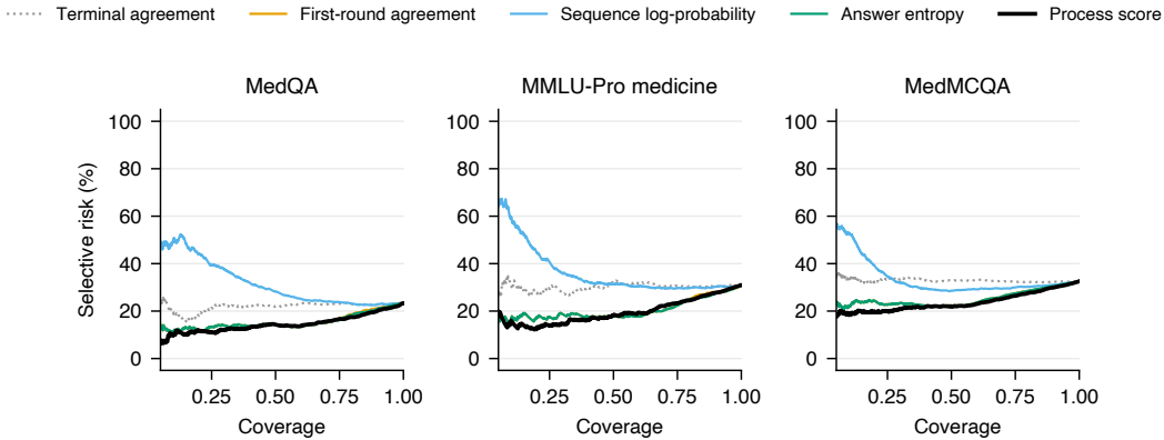
Figure 5: Risk-coverage curves of the always-available signals on the Qwen3-8B substrate; lower is better, and the AURC values of Table 2 are the areas under these curves. The process score uses the same five-fold out-of-fold protocol as the tables; coverage below 5% is omitted.
