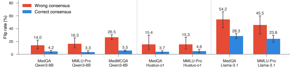
Figure 3: Flip rates of wrong and correct consensus under counter-evidence. A consensus counts as flipped when the majority vote of the N=8 re-answers no longer lands on the original answer. Flip rates per backbone and benchmark with Wilson 95% confidence intervals. The asymmetry holds in every cell, and the per-question keep rate discriminates on all seven (AUROC 0.638–0.729).
