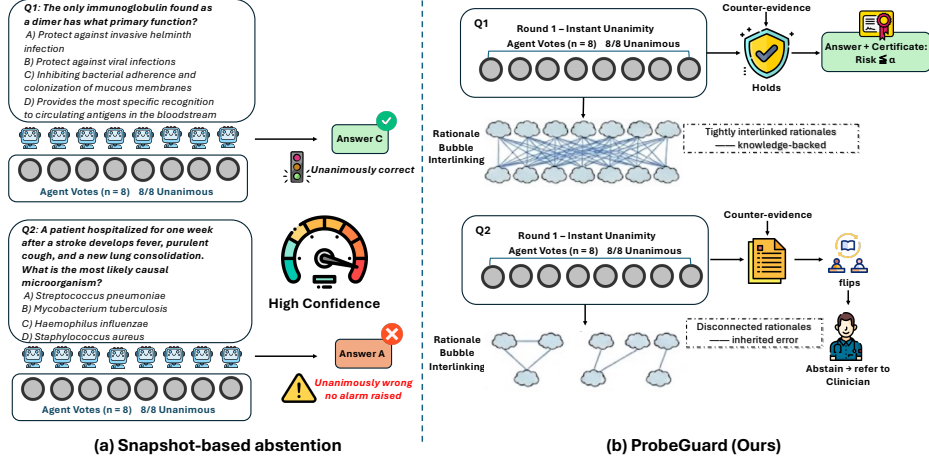
Figure 1: Two unanimous consensus are indistinguishable to snapshot-based abstention (a), yet one is knowledge-backed and one is inherited from a shared misconception. ProbeGuard (b) checks whether the rationales behind a unanimous vote support one another and stress-tests the consensus with retrieved counter-evidence, answering only where selective risk is certifiably bounded.
