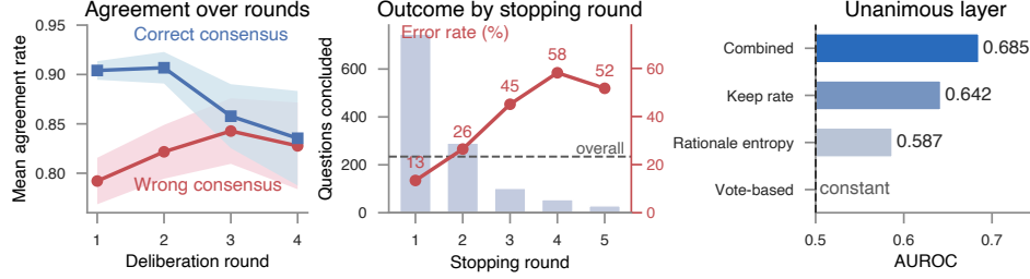
Figure 2: (Left) Correct consensus starts near-unanimous, while wrong consensus starts from disagreement and converges to it slowly (MedQA, mean agreement per round, shaded standard errors). (Middle) Error rate rises with the round at which consensus concludes (bars: questions concluding per round; line: error rate at that round; dashed: overall). (Right) On the unanimous layer every vote-based signal is constant, and only the formation signals discriminate.
