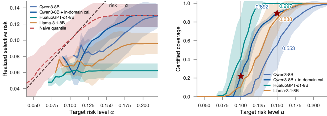
Figure 4: Realized risk and certified coverage of the stratified rule. (Left) Realized selective risk against the target level: every Learn-then-Test arm stays below the \text{risk} = \alpha diagonal at every level it certifies, while naive quantile calibration crosses it. (Right) Certified coverage per backbone on the MedQA unanimous layer; printed values are the \alpha=0.15 coverages, and stars mark the two operating points of §4.4. Lines are means over 50 calibration/test splits; bands are \pm 1 standard deviation.
