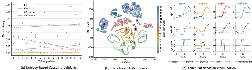
Figure 6: CATOK Produces Causal Tokens with Generative Semantics. (a) Causal Ordering CATOK’s entropy decreases in the forward order ( CATOK fwd ) and increases in the reverse order ( CATOK rev ), while FAST and Bin show weaker positional structure. (b) Token embedding geometry. T-SNE map shows slot-dependent organization, progressing from smooth early-token regions to compact late-token clusters. (c) Prefix reconstruction. Increasing token prefixes produce structured trajectory updates, with dashed curves showing incremental contributions.
