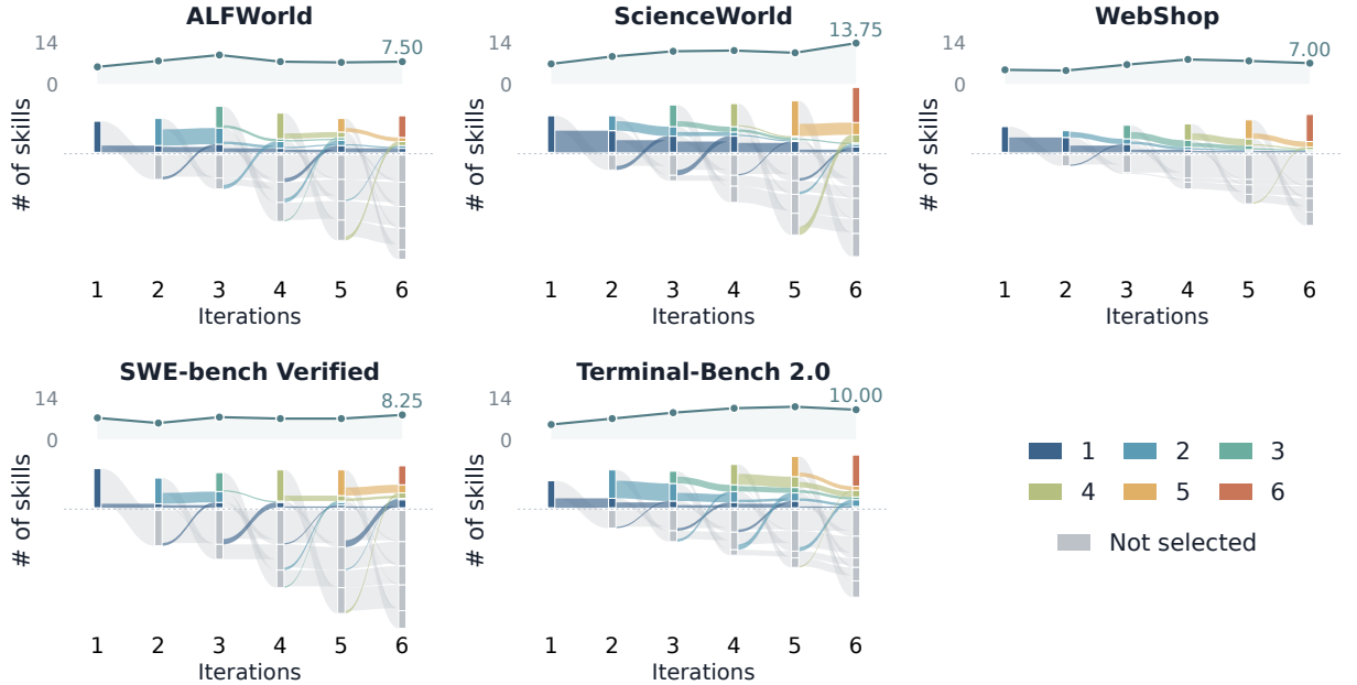
Figure 5 | RSI-router accumulates new skills while reusing experience across iterations. Upper curves show the mean number of execution skills per candidate router. Lower flows track unique skill sources across iterations.
