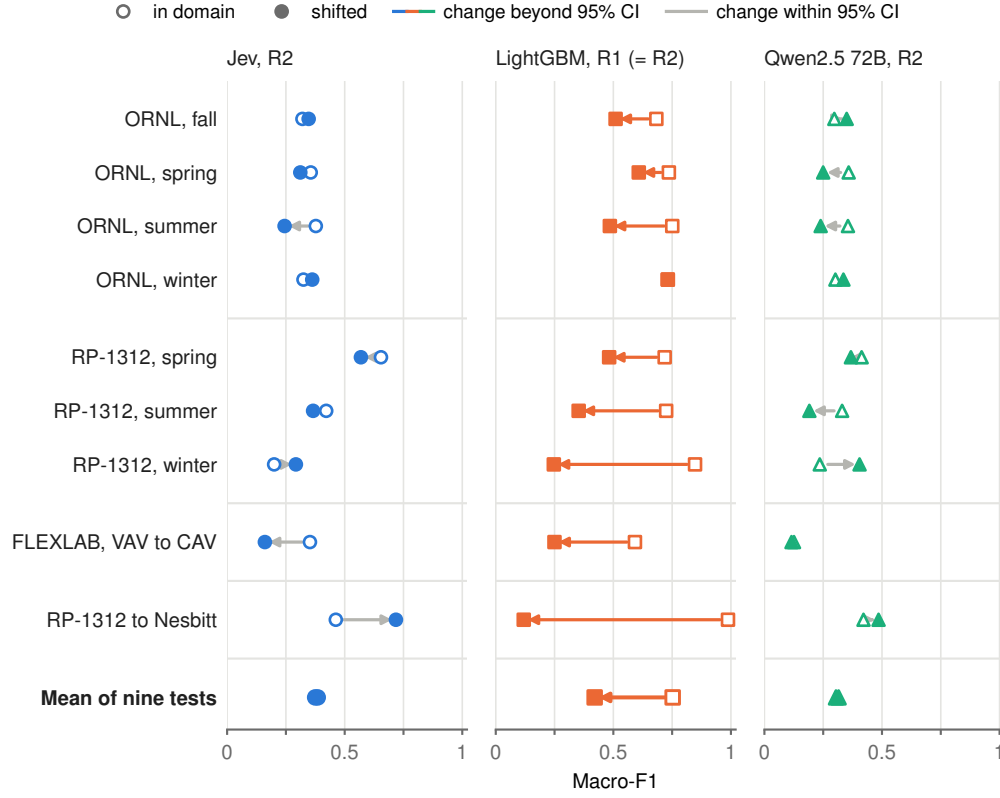
Figure 3: Macro-F1 in domain and on the shifted test set. Each arrow runs from the in-domain score to the shifted score, so its length is the loss under shift. Seasons are the held-out season. Table D.1 gives the values and intervals.
