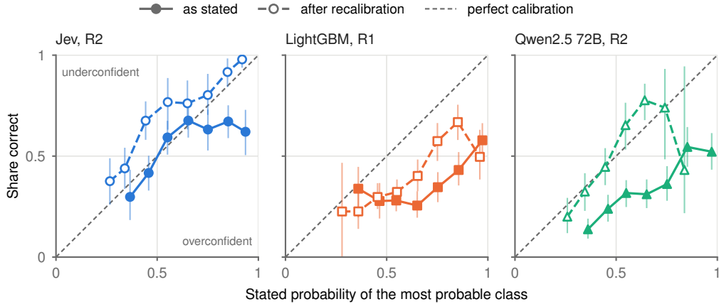
Figure 4: Reliability diagrams on the shifted test sets, pooled over the nine shift tests. Each point is a bin of windows grouped by stated probability. Bins with fewer than 30 windows are omitted.
