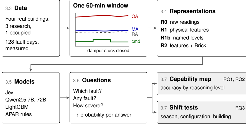
Figure 1: Study design. Numbers in the boxes are the sections that describe each step. Window values are illustrative. OA, MA, RA: outdoor-, mixed-, and return-air temperature; cmd: damper command.
