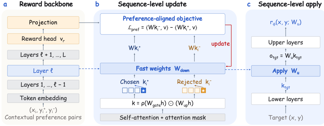
Figure 3: Overview of P-TTT.
