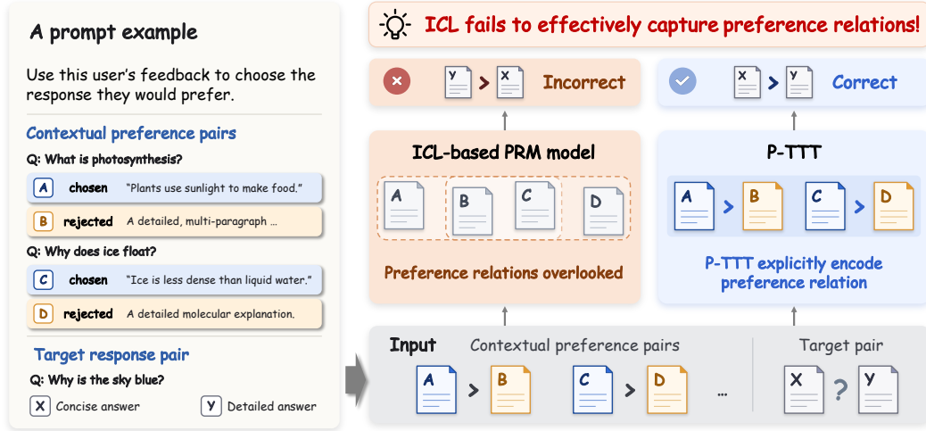
Figure 1: Illustration of personalized reward modeling with ICL and P-TTT (Ours). While an ICL-based PRM can utilize the content of contextual preference pairs, it may fail to capture their preference relations, resulting in an incorrect target prediction. P-TTT explicitly encodes these relations to better guide target response reward evaluation.
