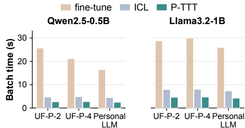
Figure 4: Inference time per batch samples for different methods.
