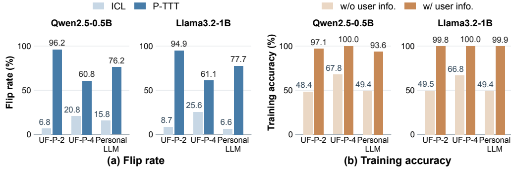
Figure 2: (a) Flip rates of ICL and P-TTT. (b) Training accuracy of ICL-based PRMs with and without contextual preference examples.
