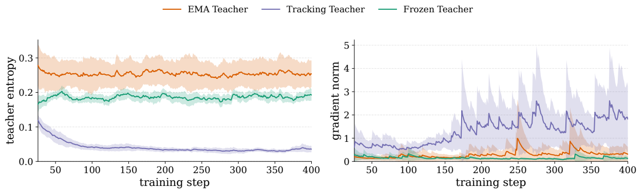
Figure 5: Teacher entropy (left) and gradient norm (right) on SciKnowEval-Physics during training under tracking, frozen, and EMA teacher updates. Lines and bands show the mean and standard deviation over three seeds.
