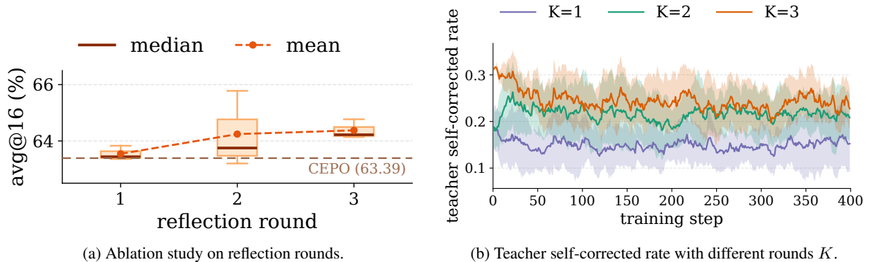
Figure 6: Reflection-round analysis for ReTeach on SciKnowEval-Physics.
