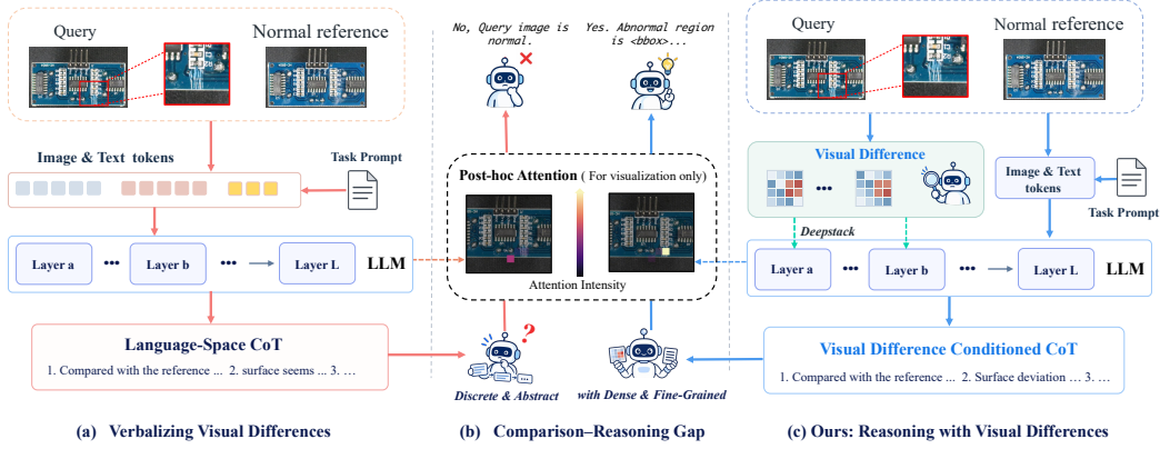
Figure 1: Verbal comparison versus visual-difference conditioning. (a,c) Two reasoning routes using the same query–reference pair. (b) Example predictions and post-hoc attention maps, shown for interpretation only and not used as model inputs.
