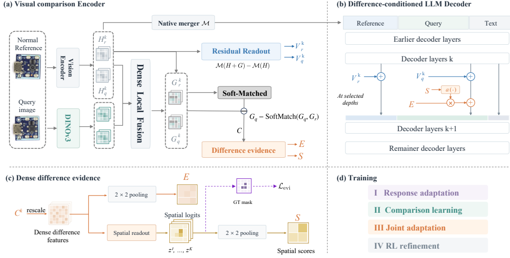
Figure 2: VD-DeepStack overview. Blue paths provide appearance context to both images; orange paths inject difference vectors E only into query tokens, weighted by spatial scores S . Injection occurs during prefill without adding tokens.
