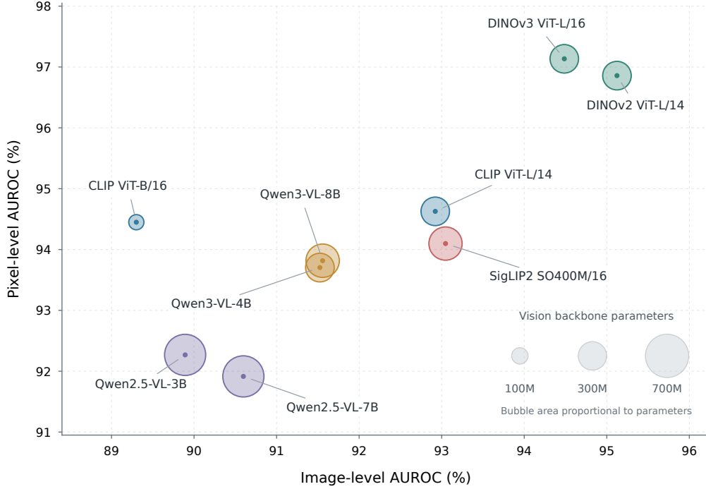
Figure 4: Frozen visual encoders under a common one-shot matching protocol. Bubble area indicates vision-backbone parameter count; Qwen labels identify the parent vision-language models.
