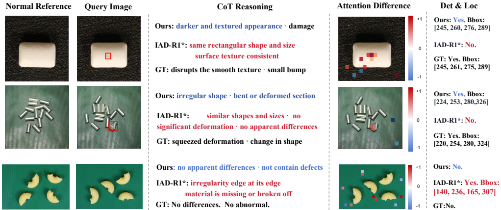
Figure 3: Qualitative comparison with IAD-R1*. Attention is extracted from the token position immediately preceding the final answer, after reasoning, to query-image tokens and averaged over the last four LLM layers. Attention differences are computed as VD-DeepStack minus IAD-R1*; red and blue indicate increased and decreased attention, respectively.
