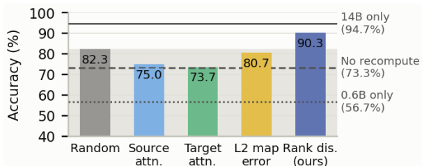
Figure 7: Selectors at a matched budget ( \rho=0.3 ), for 300 samples on GSM8K, transfer mapping Qwen3-0.6B→14B. The shaded band marks random selection.
