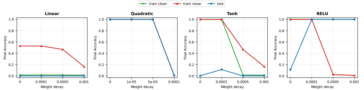
Figure 10: (a)–(d): Final accuracy using activation functions \sigma(x) = x (linear), \sigma(x) = x^2 (quadratic), \sigma(x) = \tanh(x) , or \sigma(x) = \max(0, x) (ReLU), under different weight decay.
