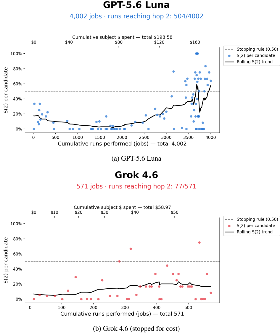
Figure 8: Second-hop survival S(2) of candidate templates over the course of the search for GPT-5.6 Luna and the frontier-class Grok 4.6. Bottom axis: cumulative jobs; top axis: cumulative target-model cost, with ticks placed at the job count where each cost was reached, so their spacing is uneven. Points are individual candidate templates and the black line is a rolling average. The dashed line marks the S(2) > 0.50 threshold of the stopping rule (Section 4.2).
