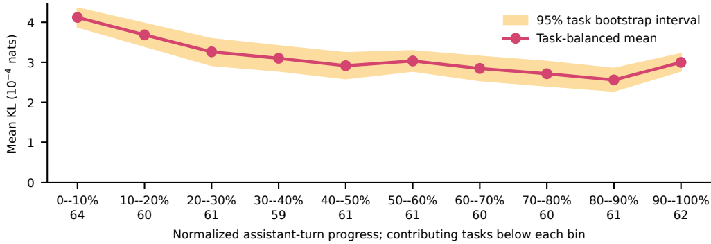
Figure 16: Distributional change across rollout progress. Task-balanced forward KL between the base and one-update Uniform policies, grouped by normalized assistant-turn progress. The band shows the 95% task-bootstrap interval. Counts below the bins give the number of contributing tasks.
