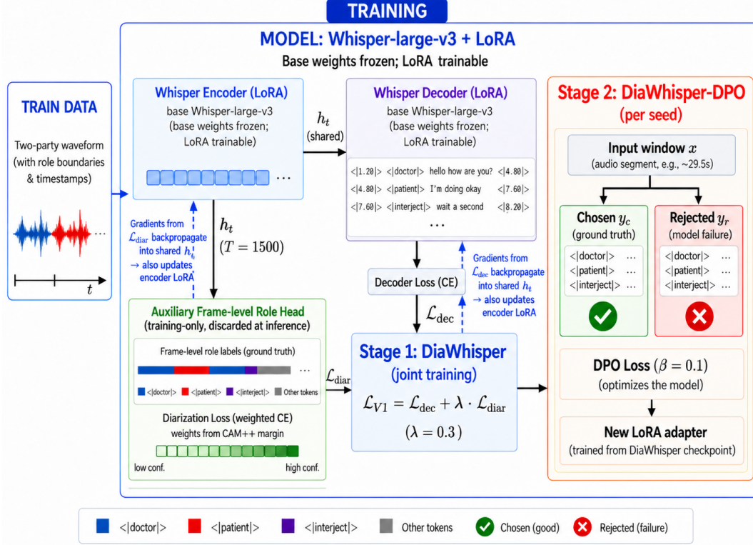
Fig. 1. Training pipeline: Stage 1 produces DiaWhisper; Stage 2 refines it into DiaWhisper-DPO. Both share the inference procedure in Section 2.4.
