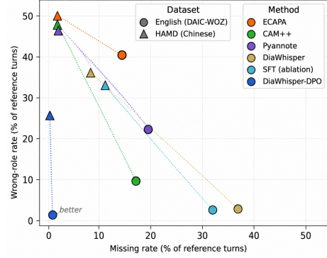
Fig. 2. Missing rate vs. wrong-role rate by method, DAIC-WOZ (circle) and PDCH-HAMD (triangle); dotted lines join each method’s two points. DiaWhisper-DPO sits closest to the origin on both datasets, nearly eliminating missing turns on PDCH-HAMD as well as DAIC-WOZ, though wrong-role attribution remains the larger residual error there.
