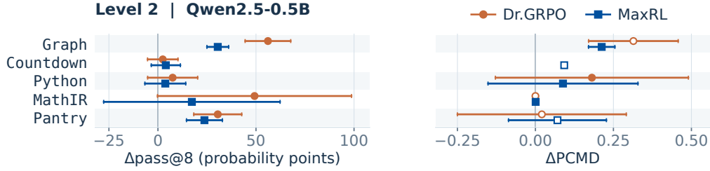
Figure 15: Replay improves Level-2 Graph accuracy and conditional solution diversity. Points show terminal Re:Dr minus Dr.GRPO and Re:Max minus MaxRL effects on pass@8 and PCMD. Bars show nominal 95% paired intervals where at least two eligible seed pairs are available.
