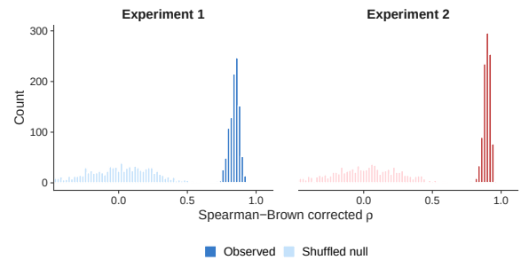
Figure 2: Split-half reliability across participants. Each panel shows the distribution of Spearman-Brown-corrected split-half correlations ( \rho ) across 1,000 random participant splits for EXP1 and EXP2. Dark bars show observed \rho values; light bars show the shuffled null distribution, in which response labels were permuted before splitting.
