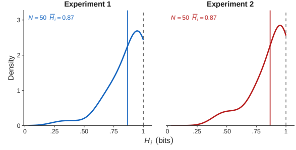
Figure 1: Distribution of item-level response entropy ( H_i , bits) across the 50 items in each experiment. Coloured vertical lines mark the per-experiment mean ( \bar{H}_i ); the dashed grey line marks the theoretical maximum ( H = 1 bit).
