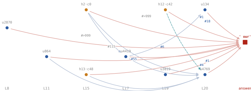
Figure 63: Qwen2.5 0.5B, predictions 1 and 2. Of 20 predictions drawn at random, these are two of the four whose sufficient set is nearest the median, 9.
