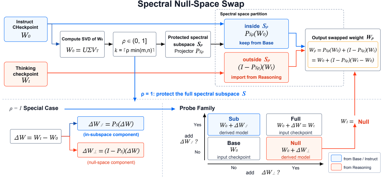
Figure 2 Overview of our method: Spectral Null-Space Swap and the \rho = 1 probe family. The swapped weight preserves the protected spectral component of the Non-thinking model and imports the complementary component of the Thinking model. The four probes isolate the contributions of \Delta W_{\parallel} and \Delta W_{\perp} .
