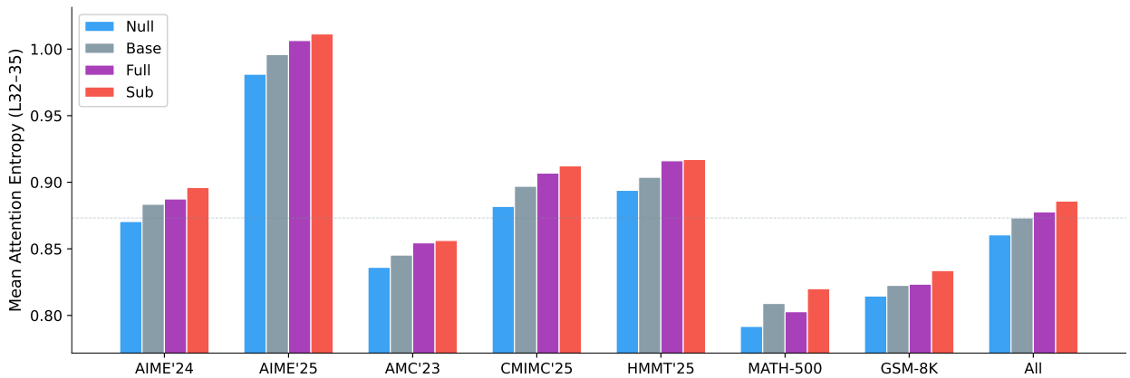
Figure 4 Layer 32–35 average attention entropy for the four variants on all seven datasets. The ordering H_{\text{Null}} < H_{\text{Base}} < H_{\text{Sub}} holds throughout; Full lies between Null and Sub in all seven datasets (values in Table 4).
