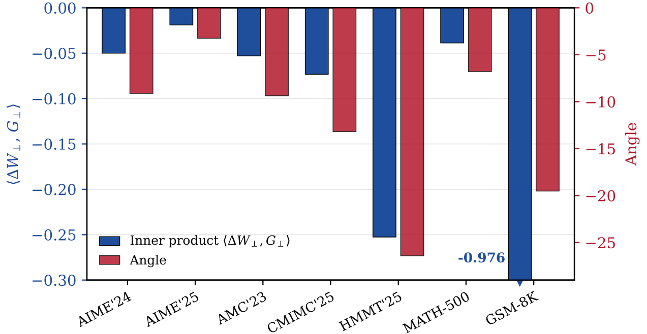
Figure 6 The null-space component negatively aligns with the entropy gradient across all benchmarks. G_{\perp} is the layer 32–35 mean attention entropy gradient at Base , and \Delta W_{\perp} is the null-space component. Left axis: inner product \langle \Delta W_{\perp}, G_{\perp} \rangle across all weight matrices, which are consistently negative. Right axis: Angle between the two vectors.
