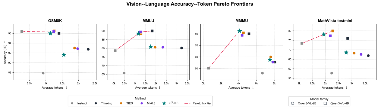
Figure 8 Accuracy–token Pareto frontiers across four vision–language benchmarks. Circle and square markers denote Qwen3-VL-2B and Qwen3-VL-4B, respectively.
