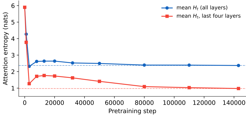
Figure 5 Attention entropy versus pretraining step (Pythia-1.4B), measured on fixed chain-of-thought input. Both curves converge to their final levels (dashed lines).
