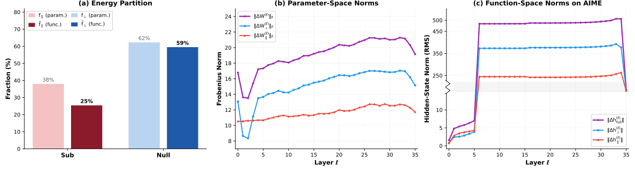
Figure 1 This figure compares the parallel and perpendicular components of the thinking difference in parameter and function spaces. All panels use the Qwen3-4B-Instruct and Qwen3-4B-Thinking. Parameter space denotes weight differences; function space denotes hidden-state offsets relative to Qwen3-4B-Instruct on AIME24/25. (a) Global average results. (b) Per-layer parameter-space results. (c) Per-layer function-space results on the same inputs.
