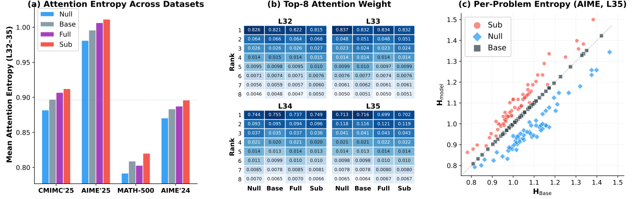
Figure 3 Attention entropy analysis across four model variants. (a) Mean attention entropy averaged over layers 32-35: Null consistently achieves the lowest entropy while Sub exhibits the highest; additional results are shown in Appendix A.2. (b) Top-8 attention weights at layers 32-35 show that Null concentrates attention. (c) Per-problem entropy scatter on AIME at layer 35: the ordering H_{\text{Null}} < H_{\text{Base}} < H_{\text{Sub}} holds for all the individual problems.
