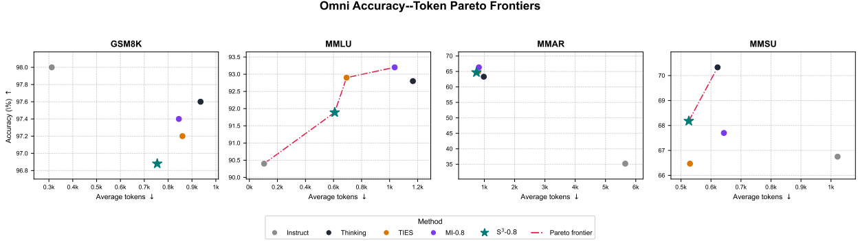
Figure 9 Accuracy–token Pareto frontiers across four Omni benchmarks.
