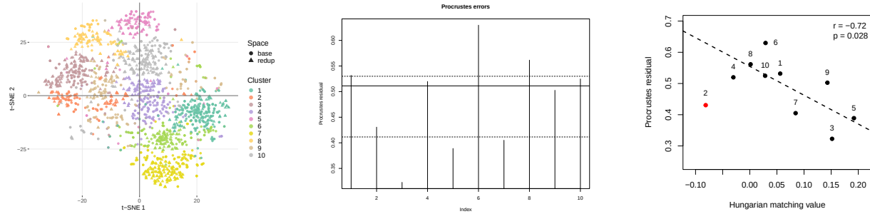
Figure 9: Procrustes analysis of the base word and reduplicative construction spaces. Left panel: two-dimensional t-SNE map of base-word vectors and Procrustes-rotated reduplication vectors. Circles indicate base words and triangles indicate reduplicative constructions. Colors indicate the cluster correspondences by Hungarian matching. Middle panel: cluster-level Procrustes residuals for the matched centroid pairs. Each vertical line represents the residual for one matched base-reduplication cluster pair after Procrustes alignment. Larger residuals indicate clusters for which the rotated reduplication centroid remains farther away from the corresponding base-word centroid, like Clusters 6, 8, 1, 10 and 4. Right panel: regression plot relating Hungarian matching values to Procrustes residuals. Each point represents one matched cluster after Hungarian matching, with the number indicating the cluster label. Cluster 2 (Cook’s distance > 2 ) was excluded from this regression plot. The negative association indicates that clusters with higher Hungarian matching values tend to have smaller Procrustes residuals after alignment ( r = -0.72 , p = .028 ).
