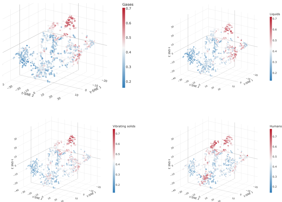
Figure 6: Three-dimensional t-SNE maps of Mandarin reduplicative constructions, with color highlighting the cosine similarity with the centroid of anchor words of Gases (top left panel), Liquids (top right panel), Vibrating Solids (bottom left panel), and Humans (bottom right panel) categories. Deeper shades of red represent higher cosine similarities, deeper shades of blue near orthogonality. An interactive version is available in the anonymized supplementary materials.
