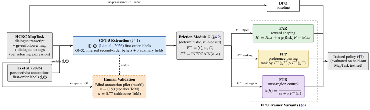
Figure 1: Pipeline overview. GPT-5 augments Li et al. (2026)’s first-order labels with second-order ToM predictions and auxiliary fields to construct the four-identifier schema. A blind human-annotation pilot audits the inferred second-order labels. The deterministic friction module \Phi computes F^- and F^+ , which condition the FAR, FPP, and FTR objectives. Standard DPO uses friction-informed preference pairs but receives no per-instance friction value; DPO-FB removes friction from pair construction entirely.
