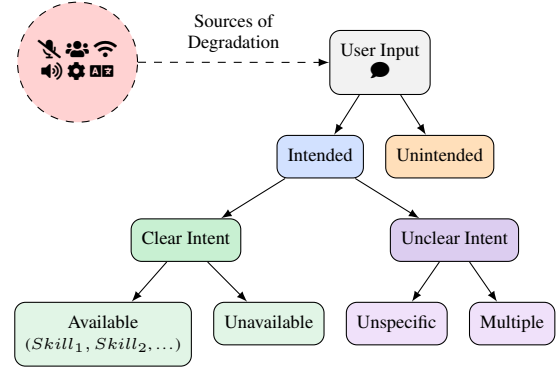
Figure 1: Classification taxonomy for fallback handling.
