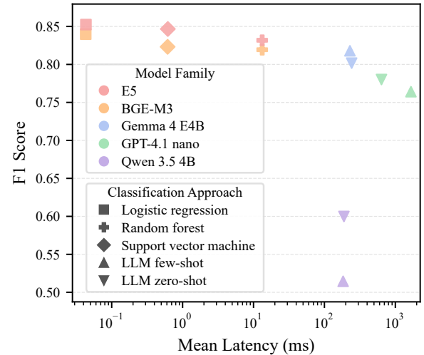
Figure 2: F1 scores of binary classification models plotted against mean latency. Colors denote model families, marker shapes denote approaches, and mean latency is shown on a logarithmic scale.
