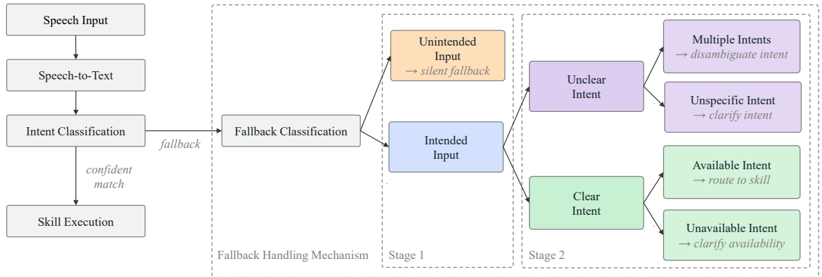
Figure 3: Hybrid fallback recovery pipeline. The intent-based dialogue manager handles matched requests; low-confidence inputs trigger a lightweight repair component consisting of a binary classification (Stage 1) and a multi-class classification for intended utterances (Stage 2). Depending on the type of the utterance, different recovery strategies are adopted.
