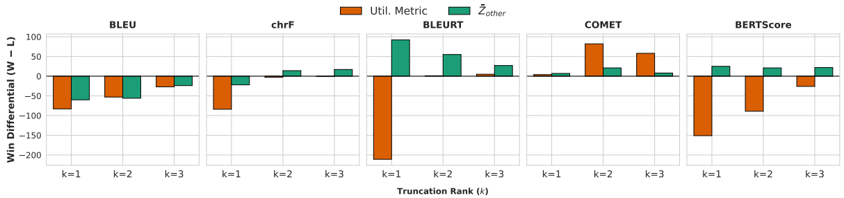
Figure 2: Sentence-level win difference (Wins – Losses) of SVD-MBR compared to the MBR for |\mathcal{Y}| = 256 . The Util. Metric is the metric used as utility function, while \bar{Z}_{other} is the mean z-score of all non-utility function evaluation metrics.
