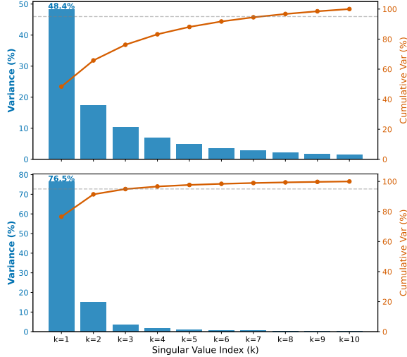
Figure 4: Cumulative variance and individual variance explained by the Top-10 singular values ( k ) for BLEU (top) and COMET (bottom) on WMT22 En→De. The grey line indicates 95% threshold.
