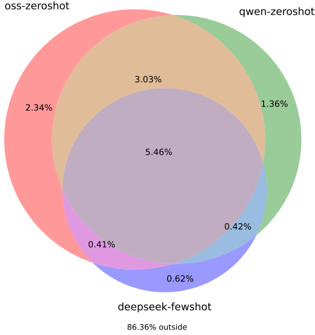
Figure 3: Token-level overlap of non-○ annotations across the three LLM-labeled test sets: GPT-OSS-120B, QWEN3-235B-A22B-INSTRUCT-2507 (zero-shot), and DEEPSEEK-V3-0324 (few-shot). Values denote percentage of total tokens.
