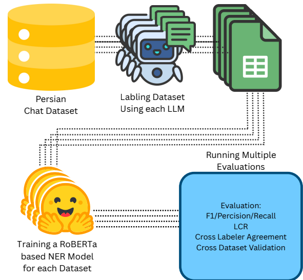
Figure 1: Overall research pipeline: from raw Persian chat data labeling by multiple LLMs to NER training and multi-stage evaluation.
