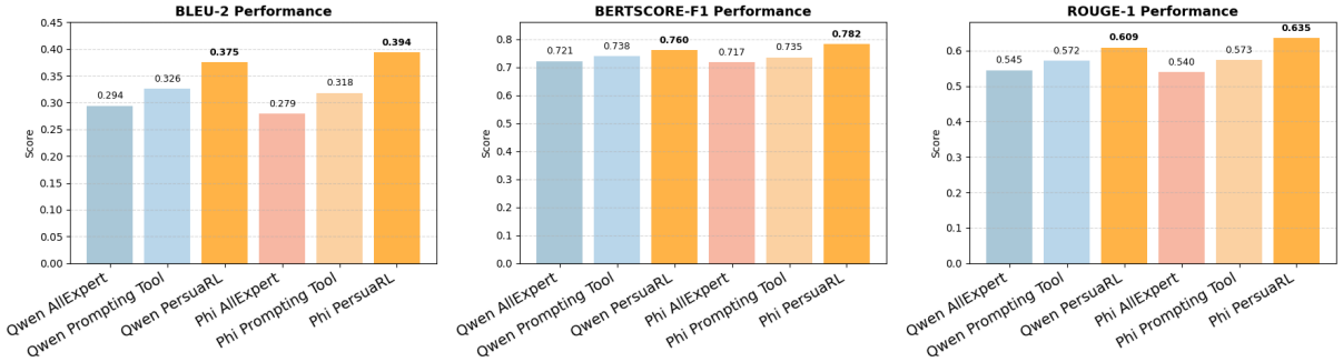
Figure 5: Ablation Study of Qwen 3B and Phi 3B variants under (a) All Tools (no selector), (b) Tools Selected via Prompting, (c) Tool Selection via Reward-Driven PersuaRL .
