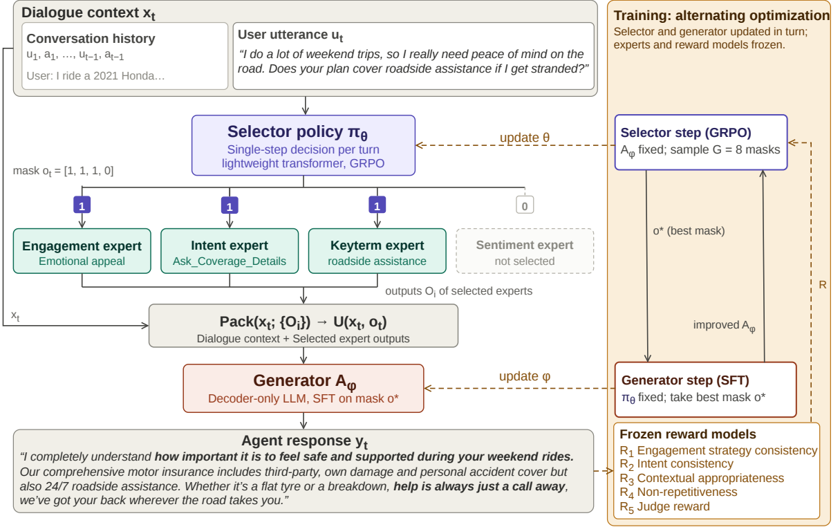
Figure 1: PersuaRL architecture with selector, generator, and reward-guided response generation. Selector and generator are trained by alternating optimization; experts and reward models are frozen. Solid arrows mark the inference path followed at every turn, dashed arrows carry training-time signals only, and the faded box denotes an expert not selected by the mask.
