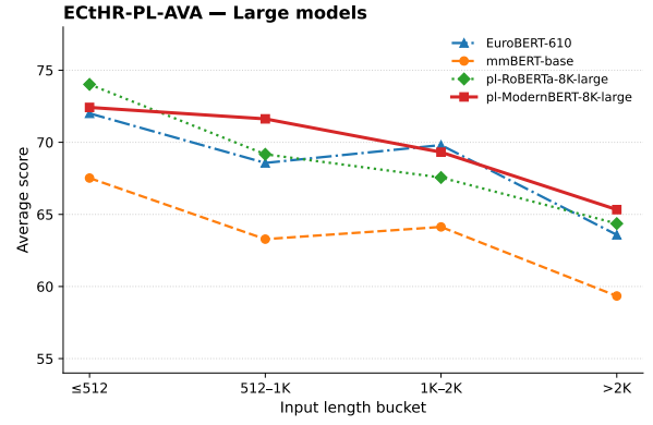
(b) ECTHR-PL-AVA: Large models.
