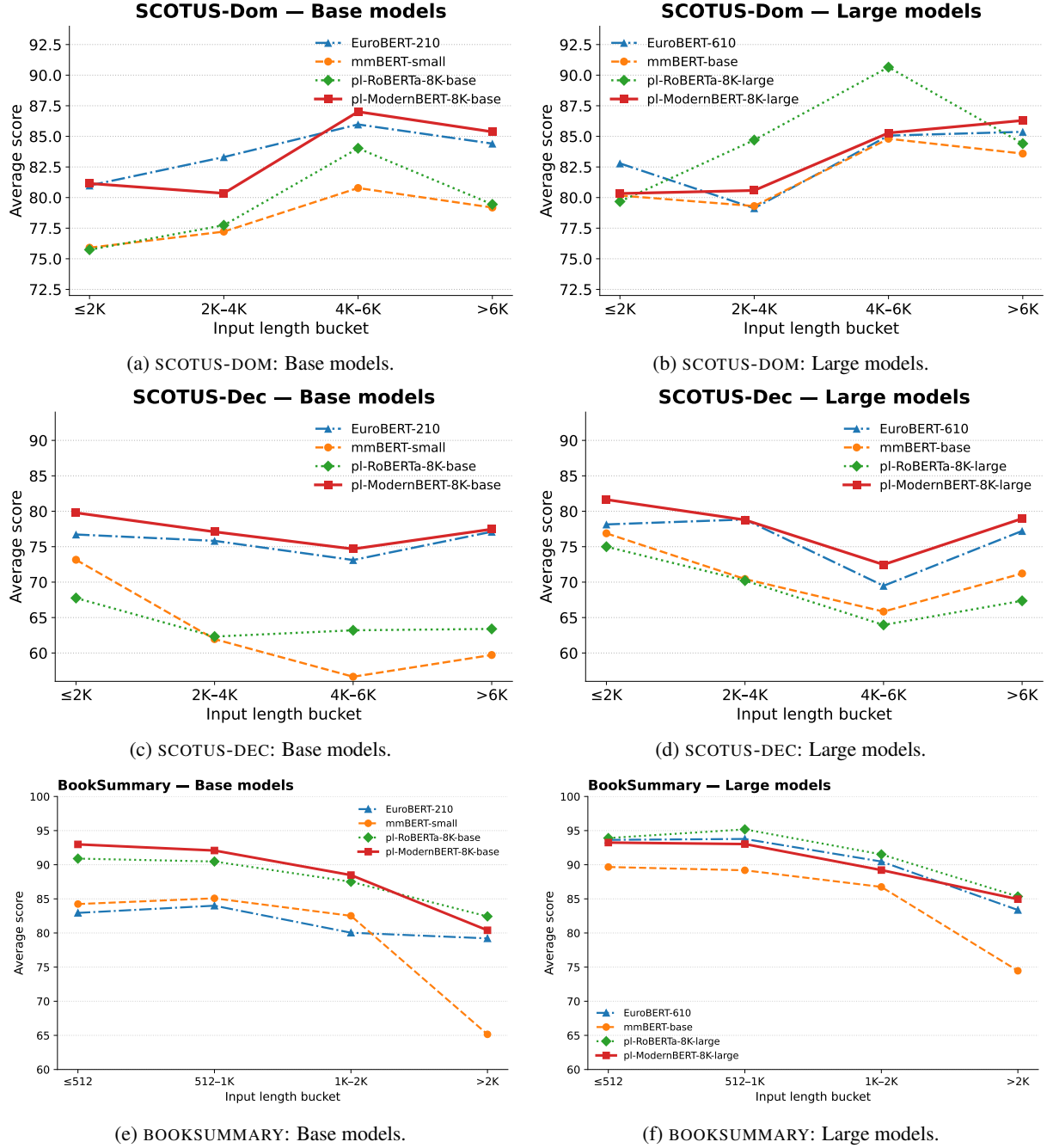
Figure 2: Performance by input length on the SCOTUS-Dom, SCOTUS-Dec, and BookSummary LongContext tasks. Each point shows the mean test score for examples within the corresponding length bucket. Results are presented separately for Base and Large models. Bucket definitions and example counts are provided in Table 14.
