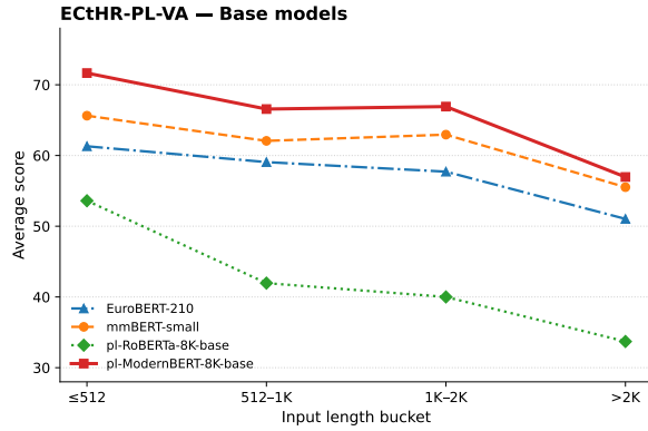
(c) ECTHR-PL-VA: Base models.
