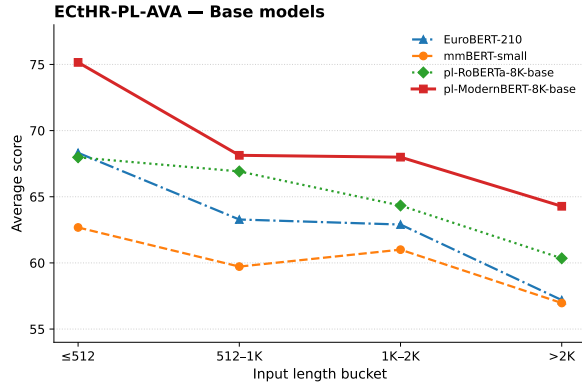
(a) ECTHR-PL-AVA: Base models.
