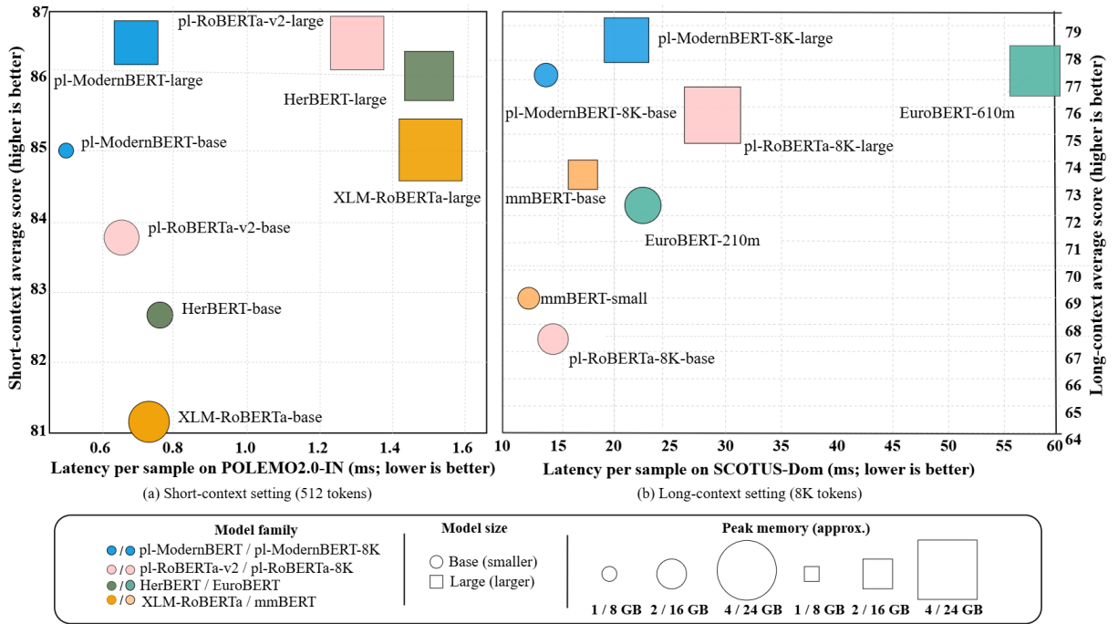
Figure 4: Quality-efficiency trade-offs for the evaluated encoder models on Polish tasks. The x-axis shows latency per sample (lower is better), the y-axis shows the average task score (higher is better), marker size reflects peak memory usage, and marker shape distinguishes Base and Large variants. Panel (a) presents short-context results, while panel (b) shows long-context results. Marker sizes are scaled separately for the two panels; slash-separated model-family names and memory labels correspond to panels (a) and (b), respectively.
