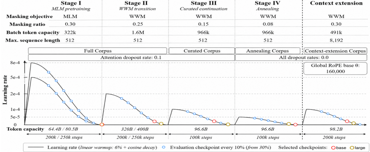
Figure 1: Polish ModernBERT pretraining schedule. The models are trained in four 512-token stages followed by 8K continuation. Blue markers denote evaluated checkpoints; red/gold markers denote selected Base/Large checkpoints. Slash-separated values correspond to Base / Large variants.
