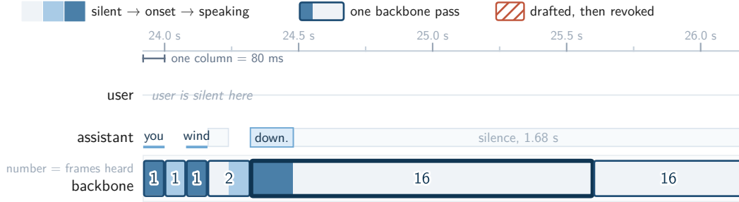
Figure 8: Long draft consumption during a stable silent interval. After several short backbone wakes, DiffuPlex-SPEAK consumes two consecutive 16-frame drafts without revision. The number inside each backbone pass indicates the number of frames realized before the next wake.
