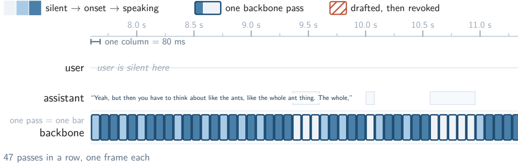
Figure 11: Repeated one-frame retention during a stable user context. Although the user remains silent, DiffuPlex-SPEAK performs 47 consecutive backbone passes that each advance only one frame. This example shows that limited acceleration can arise because the retention rule repeatedly admits only the immediate next frame, rather than because long drafts are repeatedly consumed and then revoked.
