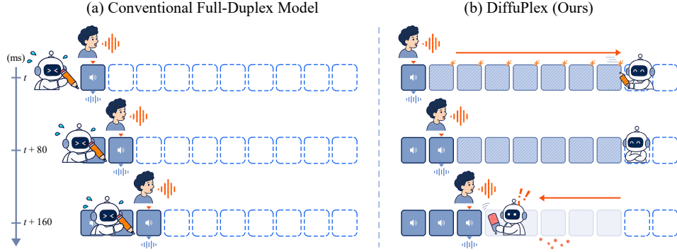
Figure 1: Overview of conventional full-duplex generation and DiffuPlex. Conventional models advance one interaction frame at a time, requiring a new backbone computation at every step (left). DiffuPlex predicts multiple future frames in a single backbone wake, consumes a retained prefix, and revises only the unplayed future when new user input diverges from the prediction (right).
