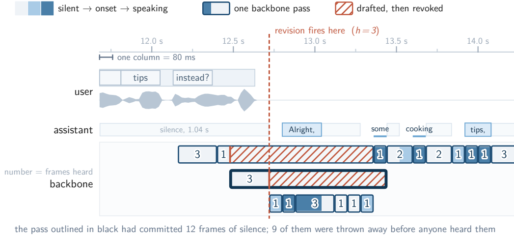
Figure 9: Revision after partial draft consumption. For DiffuPlex-SPEAK, the highlighted backbone pass drafts 12 frames of assistant silence. Revision fires after three frames have been consumed, discarding the remaining nine unplayed frames before a new assistant continuation is generated. Hatched regions denote drafted frames that are revoked before playback.
