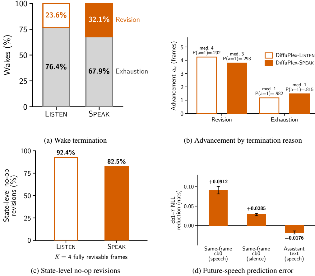
Figure 7: Rolling-draft diagnostics. Revision-triggered wakes typically occur after several frames have already been consumed, whereas exhaustion is dominated by one-frame advances. State-level no-op revisions compare the next K = 4 fully revisable frames. Positive NLL reduction indicates improved future acoustic prediction.
