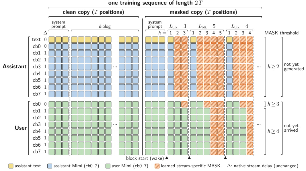
Figure 4: Training sequence layout for masked future prediction. A clean and masked copy of the same 17-stream sequence are concatenated to form a sequence of length 2T . The masked dialog region is tiled by variable-length blocks, with lookahead h reset at every block start. Inputs unavailable at that backbone wake are replaced by learned stream-specific MASK tokens: assistant streams from h \geq 2 , user cb0 from h \geq 3 , and user cb1–7 from h \geq 4 . Native stream delays are unchanged. The staircase denotes stream-wise input availability rather than an attention mask; temporal attention remains causal.
