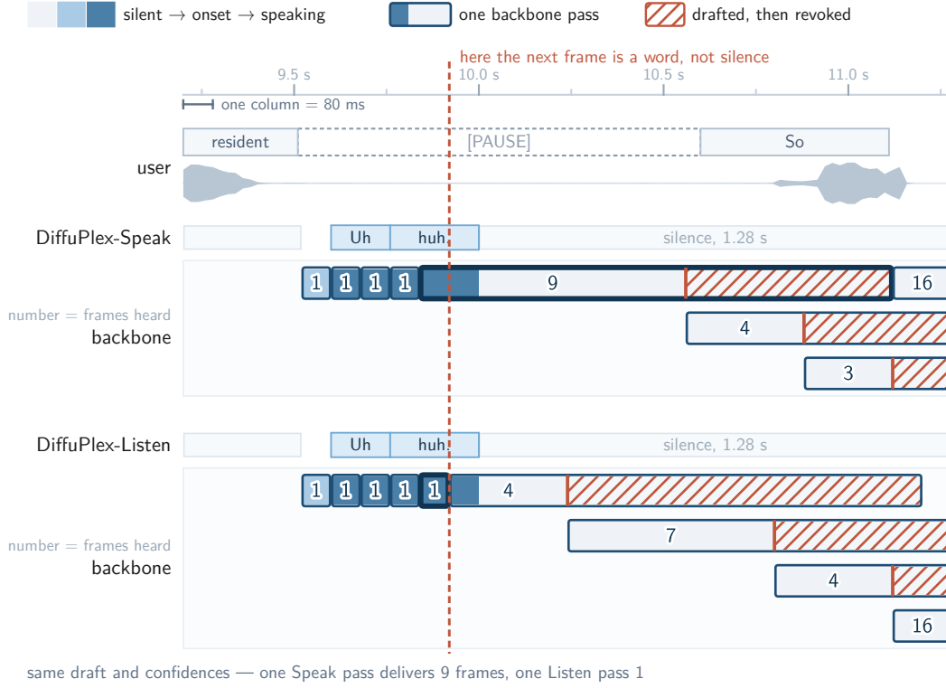
Figure 10: Different retention policies on the same interaction. Because the prediction at h = 2 is lexical, DiffuPlex-LISTEN retains only the autoregressive frame ( r = a = 1 ), whereas DiffuPlex-SPEAK retains r = 16 and consumes a = 9 before revision.
