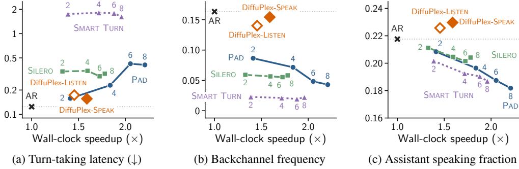
Figure 3: Efficiency-interaction trade-offs under deferred execution. Deferred baselines vary R \in \{2, 4, 6, 8\} , and deferred frames are forced to silence. Silero and Smart Turn replay precomputed controller decisions; controller inference cost is measured separately.
