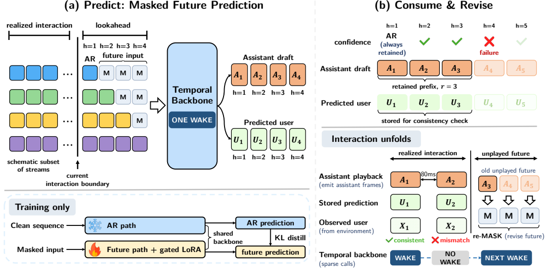
Figure 2: Overview of DiffuPlex. (a) One backbone wake predicts a masked future block with an assistant draft and user predictions. The staircase indicates stream-wise masking of inputs unavailable at that wake; the exact 17-stream layout is shown in Figure 4 in Appendix C.3. (b) A confident prefix is played at the original 80ms rate without additional backbone wakes, while incoming user frames can trigger revision of only the unplayed future.
