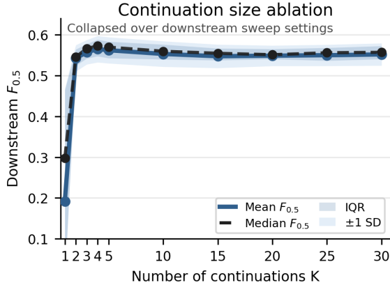
Figure 3: Continuation-sample size ablation. For each K , downstream F_{0.5} is collapsed over the decision-rule sweep. Lines show mean and median performance; shaded bands show interquartile range and \pm 1 std.
