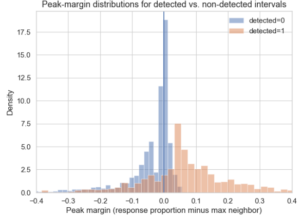
Figure 4: Distribution of peak margins for detected TRPs and non-TRP intervals. Peak margin is defined as the difference between an interval’s response proportion and the maximum of its immediate neighbors. Detected TRPs exhibit substantially larger positive margins, while non-TRP intervals are centered near zero, indicating that the labeling procedure selects positions with locally elevated listener response rates.
