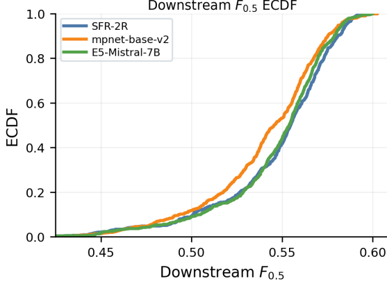
Figure 2: Distribution of F_{0.5} across the fixed- K semantic-uncertainty sweep. Each curve is an empirical cumulative distribution over configurations for one embedding model. Mean \pm SD across configurations: SFR-2R = 0.547 \pm 0.033 , all-mpnet-base-v2 = 0.540 \pm 0.033 , E5-Mistral-7B-Instruct = 0.546 \pm 0.031 .
