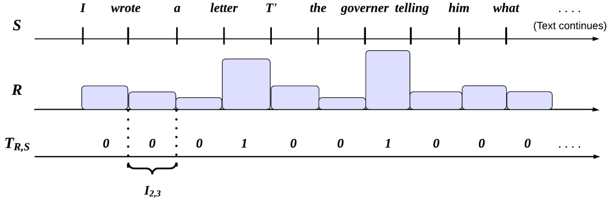
Figure 1: Schematic illustration of empirical within-turn TRP labeling. S denotes the speaker’s word sequence, R denotes aggregated listener response distribution, and T_S denotes the resulting binary reference labels. Participant response onsets are aligned to word-adjacent intervals I_{i,i+1} , each corresponding to the position following prefix P_i . Intervals are labeled positive when their empirical response proportion I_{i,i+1}^{Proportion} exceeds the stimulus-specific threshold. The example text is adapted from Schegloff (1982); the figure is inspired by Umair et al. (2024).
