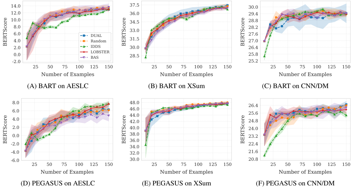
Figure 3: Number of labeled instances vs. rescaled BERTScore. Comparison of active strategies using BART and PEGASUS backbones on AESLC, XSum, and CNN/DM datasets.
