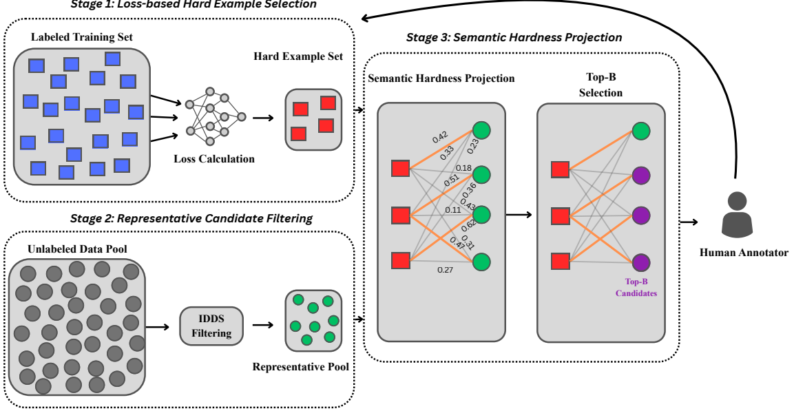
Figure 1: The three-stage pipeline of LOBSTER. (1) Loss-based Hard Example Selection identifies “Hard Example” set \mathcal{H} (red squares) via high cross-entropy loss to serve as semantic anchors. (2) Representative Candidate Filtering uses IDDS to distill a pool of representative candidates (green circles) from the unlabeled set \mathcal{U} . (3) Semantic Hardness Projection computes the Max-Similarity Score S(x_u) (Eq. 3) using Sentence-BERT embeddings. This helps to identify a “semantic twin” for each hard example, forming the final Top- B batch for annotation.
