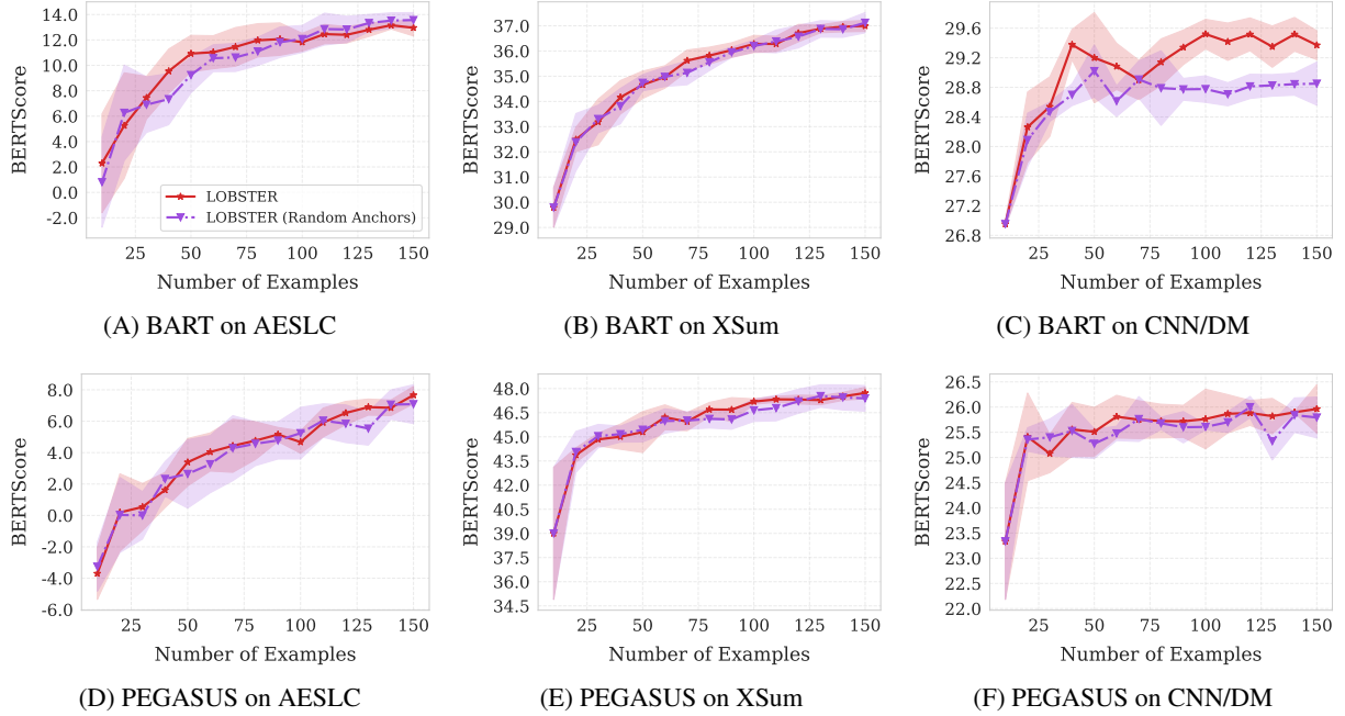
Figure 5: Number of labeled instances vs. BERTScore. Comparison of LOBSTER and the LOBSTER (Random Anchors) ablation using BART and PEGASUS backbones on AESLC, XSum, and CNN/DM datasets.
