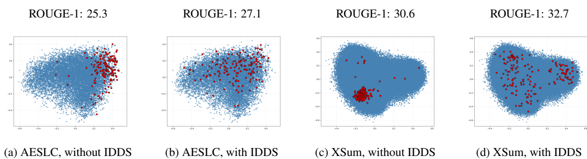
Figure 6: Impact of IDDS on Selection Diversity (PCA visualization of selected instances). Comparison of the proposed LOBSTER method with IDDS versus the ablation without IDDS. The IDDS module prevents semantic collapse by filtering redundant candidates, leading to higher ROUGE-1 scores.
