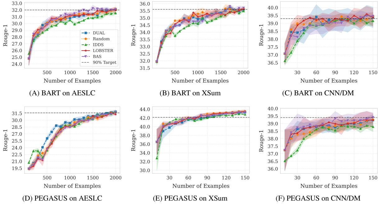
Figure 4: Number of labeled instances vs. ROUGE-1. Comparison of active learning strategies using BART and PEGASUS backbones on AESLC, XSum, and CNN/DM datasets. The dashed horizontal line in each subplot denotes the 90% performance threshold of the full-dataset baseline.
