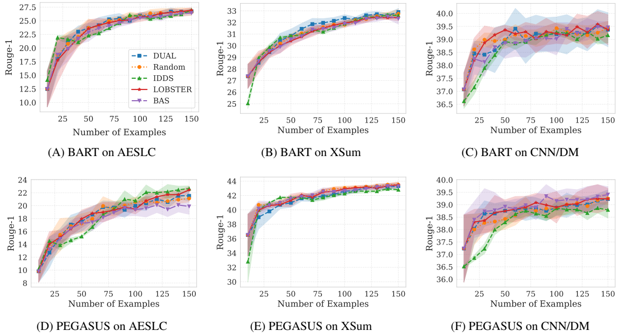
Figure 2: Number of labeled instances vs. ROUGE-1. Comparison of active strategies using BART and PEGASUS backbones on AESLC, XSum, and CNN/DM datasets.
