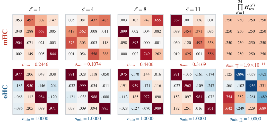
Figure 4 Illustration of H_{\text{res}} . Each cell is the 4 \times 4 residual matrix a trained model computed for a single token of the evaluation set, read from the checkpoint. Left four columns: four sublayers at depths \ell = 1, 4, 8, 11 ; right column: the product over all 24 sublayers. Top row mHC, bottom row oHC. The entry sublayer is excluded.
