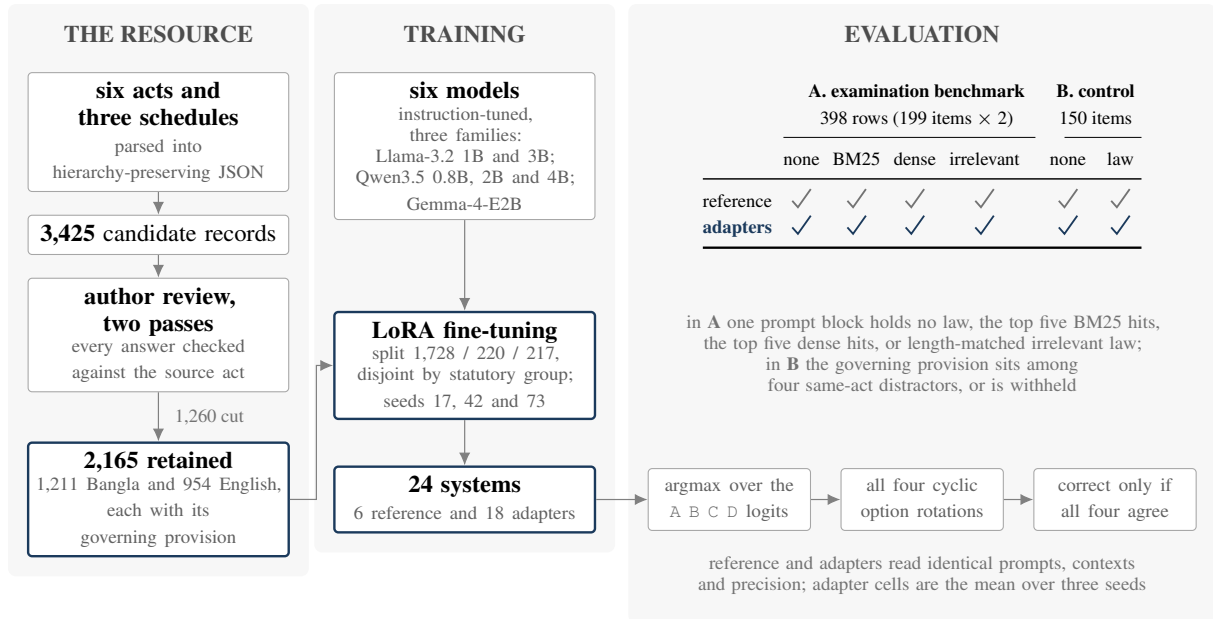
Figure 1: Study design. Panel B places the governing provision in the prompt, removing retrieval failure. The scoring chain then reads the answer from the option-letter logits, removing format from the measurement, and keeps it only if it survives all four option orders. A tick marks each executed arm.
