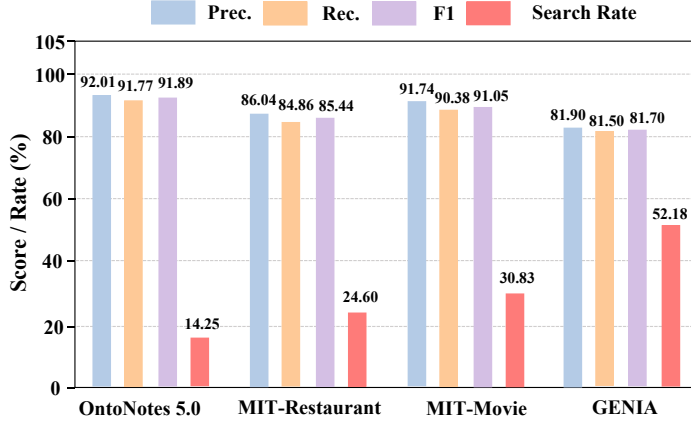
(a) Domain-wise performance and search behavior of NE-R1.
