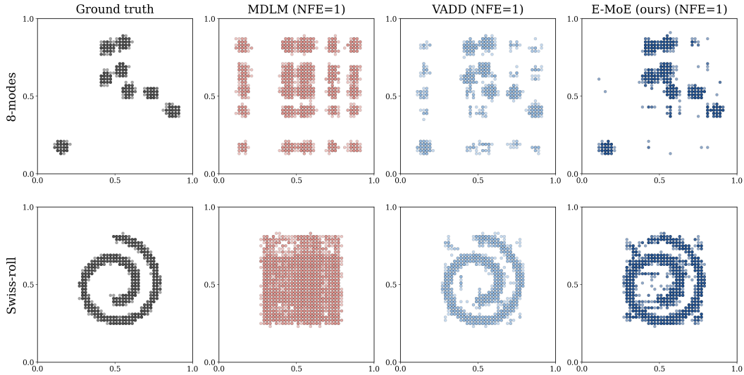
Figure 4: Generation results on 2-D toy examples. Ground truth and generations of MDLM (Sahoo et al., 2024), VADD (Xie et al., 2026), and E-MoE at NFE = 1 on 8-modes and swiss-roll. Full sweeps over \text{NFE} \in \{1, 2, 8, 32\} are in Appendix C.1.
