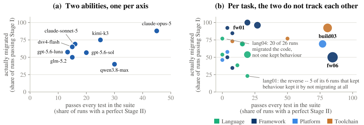
Figure 3 (a) Where each model sits on two axes, both of them shares of the same runs: horizontally “does it still behave like the original” (a perfect Stage II), vertically “was the migration done at all” (Stage I). (b) The same two axes, per task, with marker area the number of accepted submissions. A migration has to satisfy both conditions, but they are satisfied by different runs, and most runs manage at most one.
