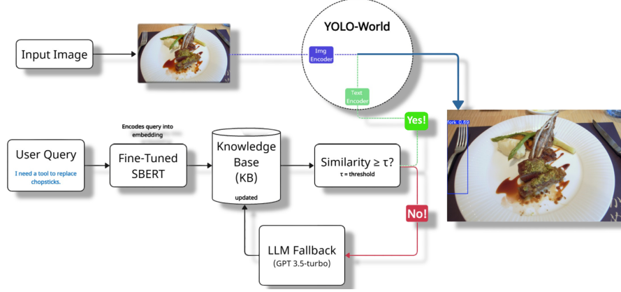
Fig. 1. Architecture of the proposed Vague2Detect pipeline. Given a vague query such as “I need a tool to replace chopsticks,” the system encodes the prompt with a fine-tuned SBERT model and retrieves the closest entry from the Knowledge Base (KB). If the retrieved object (e.g., fork) is above the similarity threshold \tau , its label is passed to YOLO-World for visual grounding. If no suitable KB match is found (for instance, if fork is not present in the KB), a GPT-based fallback generates a new candidate description for fork, which is then added to the KB and verified by YOLO-World before being accepted. This hybrid design enables the system to handle direct labels, functional queries, and novel objects while ensuring that all detections remain visually grounded.
