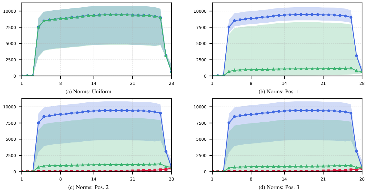
Figure 16: Layer-wise averaged hidden-state norms in Qwen2-7B for repeated-token sequences under different distinct-token positions (colors and markers as in Figure 5). The horizontal axis shows the layer index in every panel.
