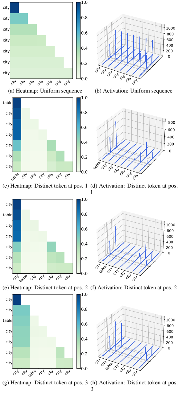
Figure 8: Results for sequences with repeated tokens. Each row compares the attention heatmap (left) and hidden-state activations (right) under the same token distribution pattern for Llama-2-7b-hf (Sample 2).
