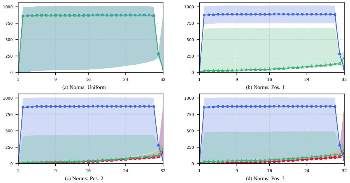
Figure 10: Layer-wise averaged hidden-state norms in Llama-2-7b-hf for repeated-token sequences under different distinct-token positions (colors and markers as in Figure 5). The horizontal axis shows the layer index in every panel.
