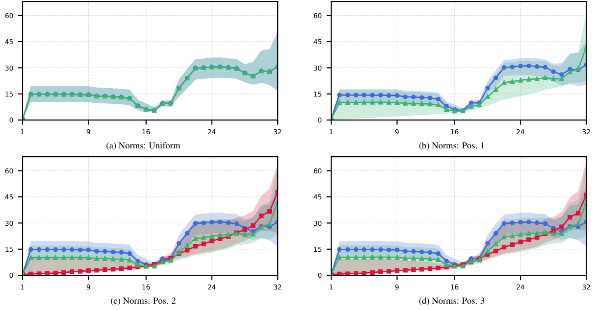
Figure 13: Layer-wise averaged hidden-state norms in Mistral-7B-v0.3 for repeated-token sequences under different distinct-token positions (colors and markers as in Figure 5). The horizontal axis shows the layer index in every panel.
