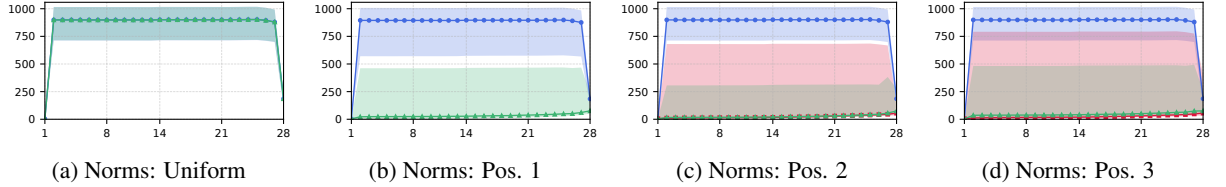
Figure 5: Layer-wise averaged hidden-state norms in Llama-3.2-3B for repeated-token sequences ( T = 64 , without a BOS token and without any attention intervention), averaged over N = 100 sequences per panel. Panels correspond to the four input patterns: a uniform repeated-token sequence (Uniform) and sequences with a single distinct token inserted at the first, second, or third position (Pos. 1–3). Blue circles and green triangles denote the first token and the mean over all remaining input tokens, respectively. Red squares denote the distinct token, and therefore appear only in the Pos. 2 and Pos. 3 panels: the Uniform panel contains no distinct token, and in Pos. 1 the distinct token is the first token itself. The horizontal axis shows the layer index in every panel. Shaded bands show the sample min–max range.
