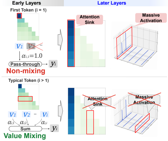
Figure 1: Main finding of this study. While attention outputs for standard tokens ( i > 1 ) are computed based on weighted averages (i.e., “mixing”) of Value vectors, the output for the initial token is based solely on its own “unmixed” Value vector. This “Value-non-mixing” state in early layers is a contributing factor in AS and MAs at the initial position of a sequence, regardless of the token occupying it.
