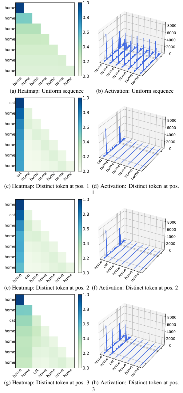
Figure 15: Results for sequences with repeated tokens. Each row compares the attention heatmap (left) and hidden-state activations (right) under the same token distribution pattern for Qwen2-7B (Sample 1).
