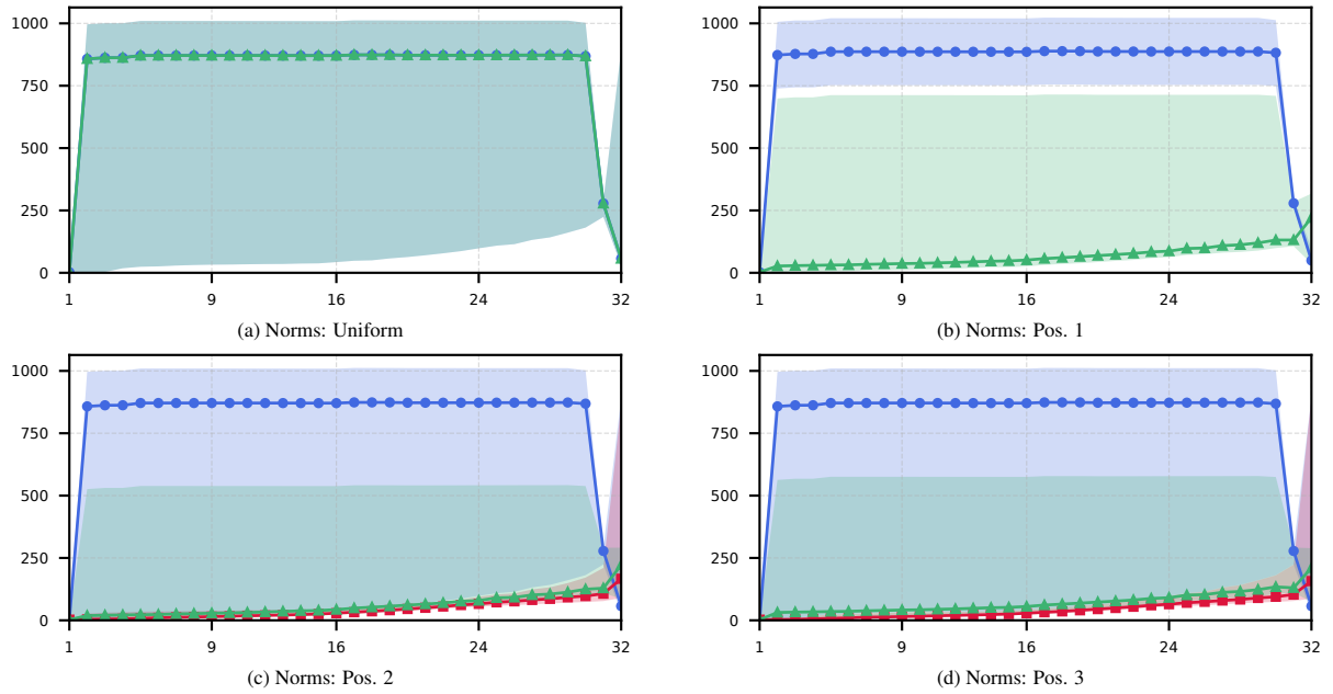
Figure 21: Layer-wise averaged hidden-state norms in Llama-2-7b-hf for repeated-token sequences of length 128 under different distinct-token positions (colors and markers as in Figure 10). The horizontal axis shows the layer index in every panel.
