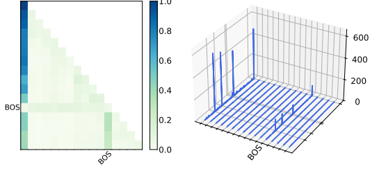
Figure 2: Attention heatmap (left) and activation magnitudes (right) from Layer 14 of Llama-3.2-3B with the BOS token swapped with the token at the 12th position of a 16-token sequence (shorter than the setting in Table 1 for readability). Both AS and MAs emerge at the initial position, independent of the BOS token location.
