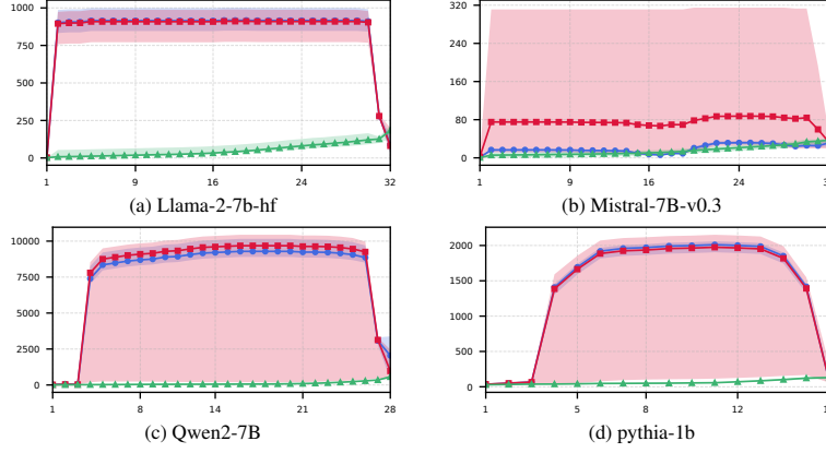
Figure 6: Layer-wise averaged hidden-state norms under the self-concentration intervention (w/o BOS token) for the four models other than Llama-3.2-3B. Blue circles, red squares, and green triangles denote the first token, the intervention token, and the mean over all other input tokens, respectively. The horizontal axis shows the layer index in every panel. Shaded bands show the sample min-max range.
