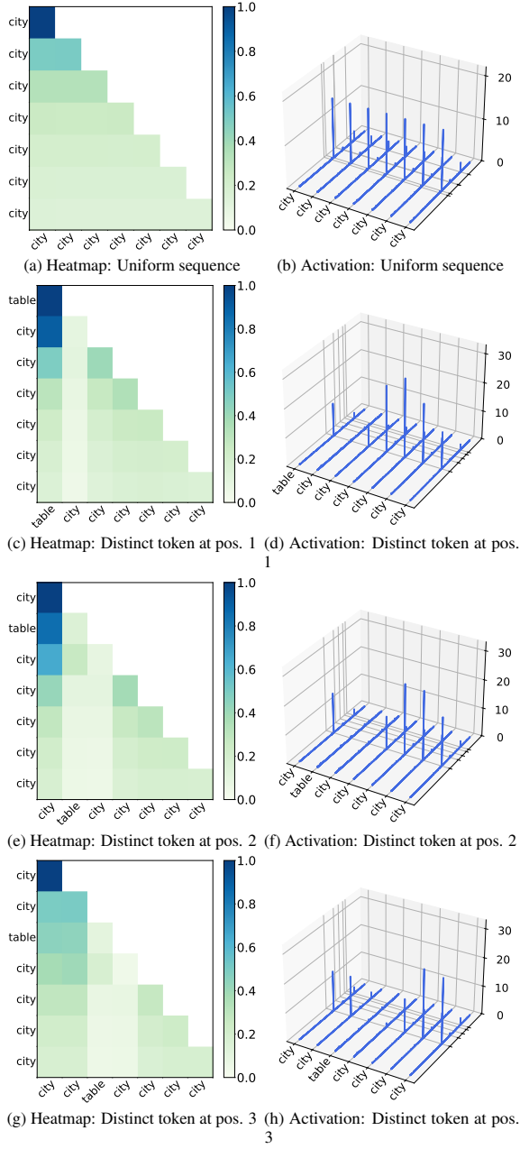
Figure 11: Results for sequences with repeated tokens. Each row compares the attention heatmap (left) and hidden-state activations (right) under the same token distribution pattern for Mistral-7B-v0.3 (Sample 2).
