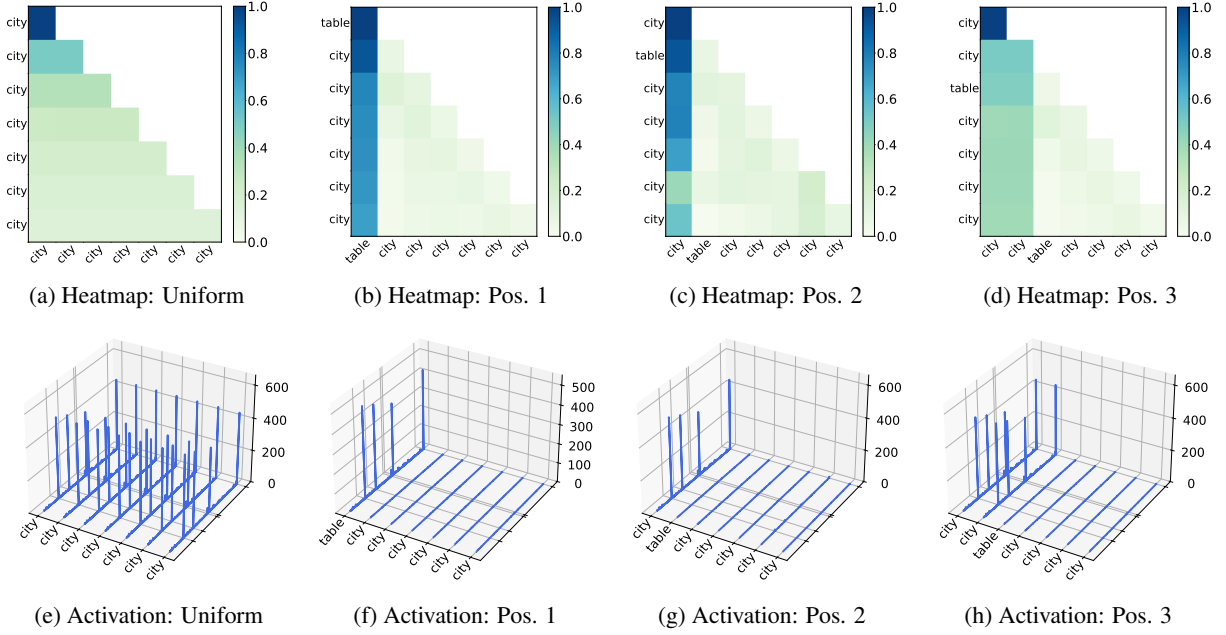
Figure 4: Attention heatmap (top row) and hidden-state activations (bottom row) at Layer 14 of Llama-3.2-3B for repeated-token sequences with varying distinct token positions.
