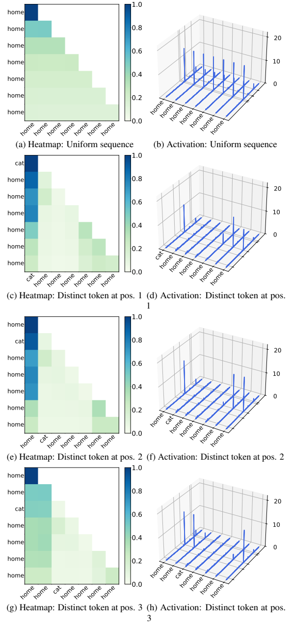
Figure 12: Results for sequences with repeated tokens. Each row compares the attention heatmap (left) and hidden-state activations (right) under the same token distribution pattern for Mistral-7B-v0.3 (Sample 1).
