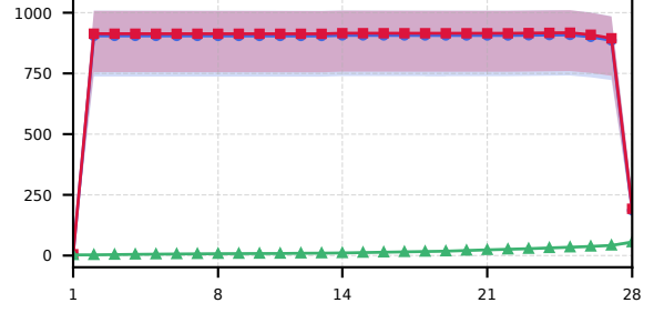
Figure 3: Layer-wise averaged hidden-state norms for Llama-3.2-3B under the self-concentration intervention (w/o BOS token). Blue circles, red squares, and green triangles denote the first token, the intervention token, and the mean over all other input tokens, respectively. The horizontal axis shows the layer index. Shaded bands show the sample min-max range.
