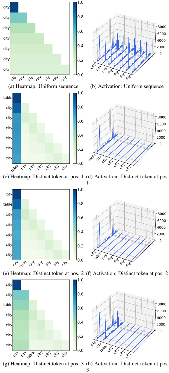
Figure 14: Results for sequences with repeated tokens. Each row compares the attention heatmap (left) and hidden-state activations (right) under the same token distribution pattern for Qwen2-7B (Sample 2).
