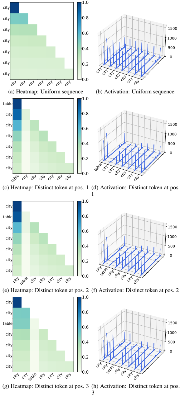
Figure 17: Results for sequences with repeated tokens. Each row compares the attention heatmap (left) and hidden-state activations (right) under the same token distribution pattern for pythia-1b (Sample 2).
