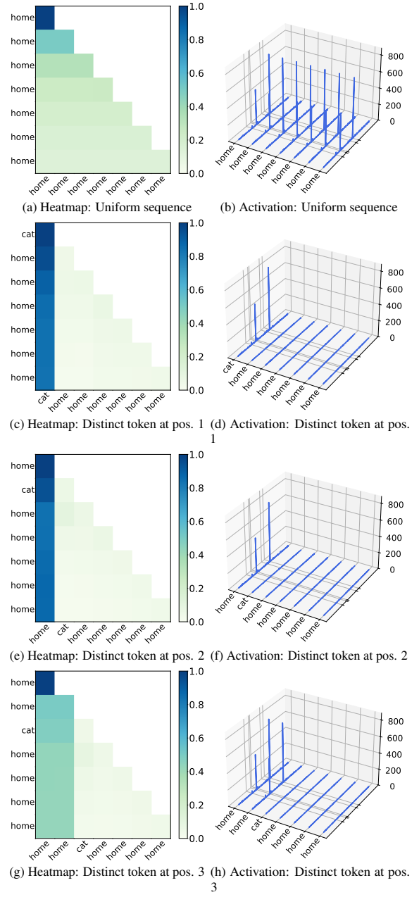
Figure 9: Results for sequences with repeated tokens. Each row compares the attention heatmap (left) and hidden-state activations (right) under the same token distribution pattern for Llama-2-7b-hf (Sample 1).
