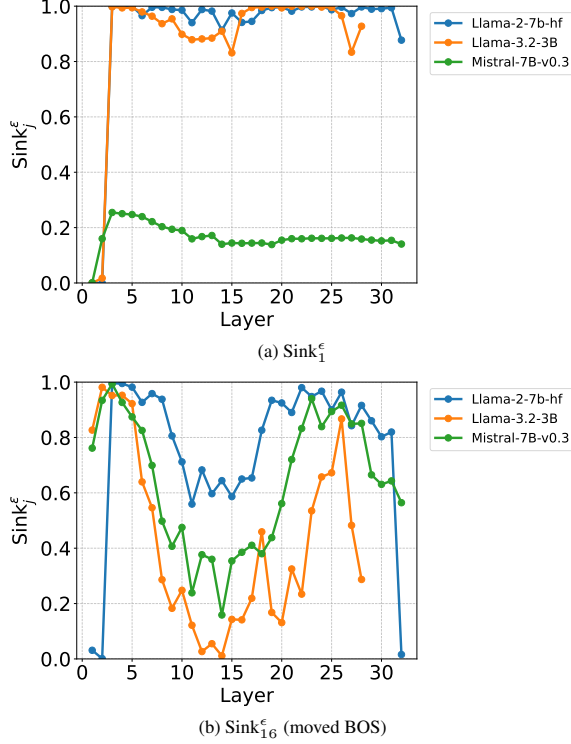
Figure 7: Transition of layer-wise \text{Sink}_j^\epsilon when the BOS token is swapped with the token at position 16 (the setting of Table 1).
