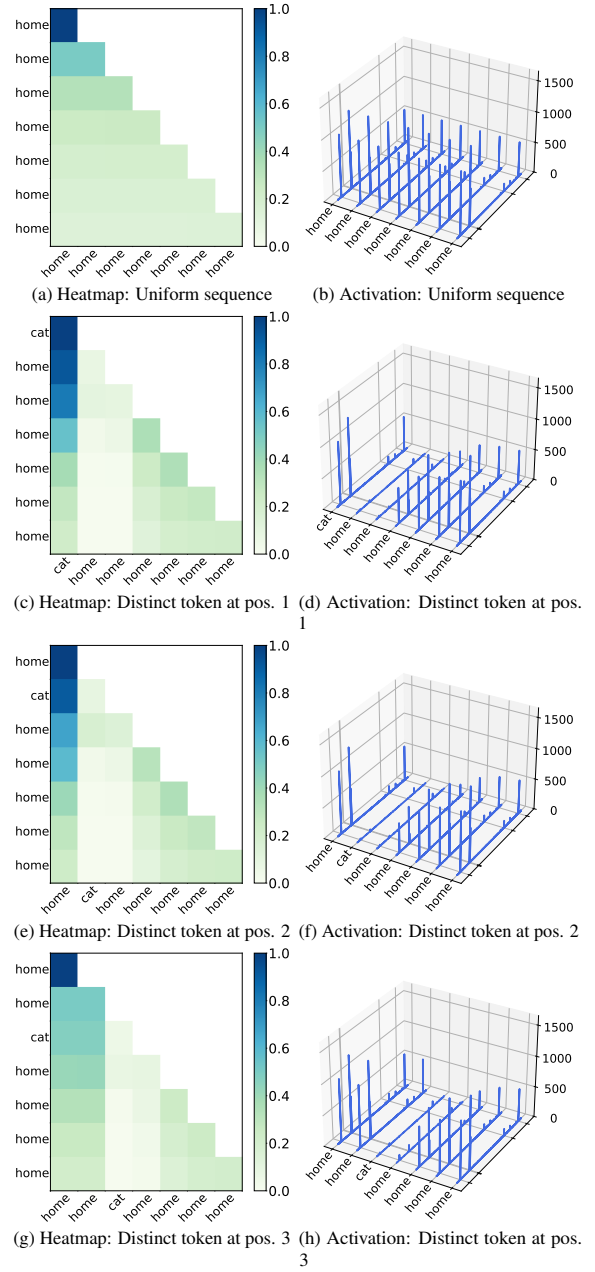
Figure 18: Results for sequences with repeated tokens. Each row compares the attention heatmap (left) and hidden-state activations (right) under the same token distribution pattern for pythia-1b (Sample 1).
