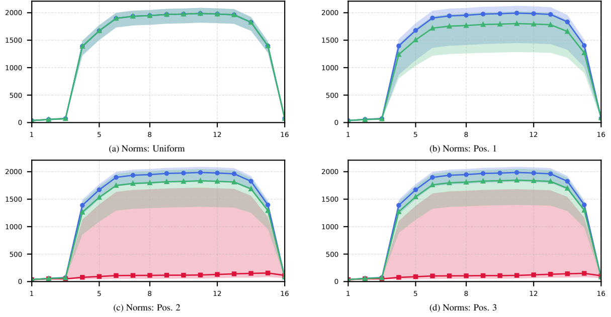
Figure 19: Layer-wise averaged hidden-state norms in pythia-1b for repeated-token sequences under different distinct-token positions (colors and markers as in Figure 5). The horizontal axis shows the layer index in every panel.
