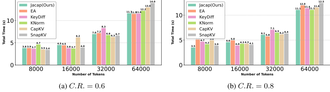
Figure 5: Runtime comparison of generating 100 tokens with Qwen3-8B on a single RTX 6000 GPU under varying input context lengths and compression ratios (C.R.)
