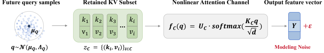
Figure 1: Nonlinear retained attention channel. A retained KV subset \mathcal{Z}_C defines a nonlinear softmax attention map from future queries q \sim \mathcal{N}(\mu_Q, \Lambda_Q) to output features, Y_C = f_C(q) + \epsilon .
