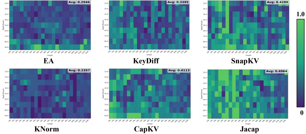
Figure 3: Performance of JACAP and baseline KV-cache eviction methods on the Needle-in-Haystack (NIAH) benchmark at compression ratio 0.75 using Qwen3-8B.
