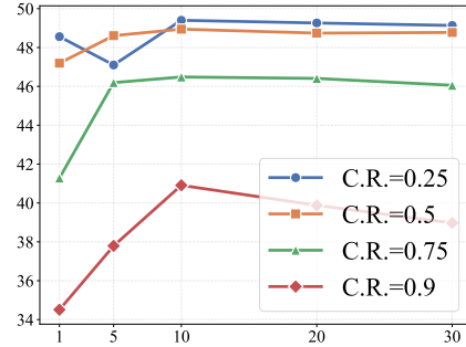
Figure 4: Ablation study of the temperature parameter \tau on LongBench.
