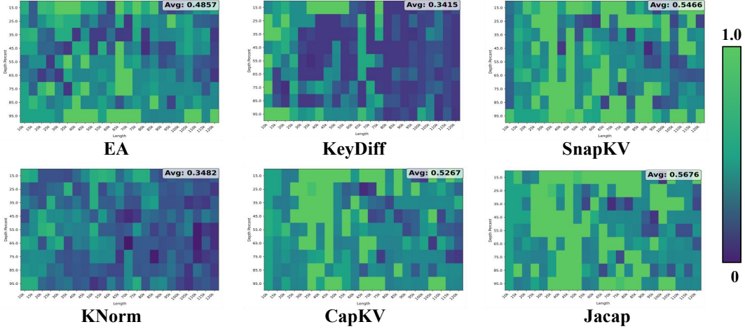
Figure 6: Performance of JACAP and baseline KV-cache eviction methods on the NIAH benchmark at compression ratio 0.5 using Qwen3-8B.
