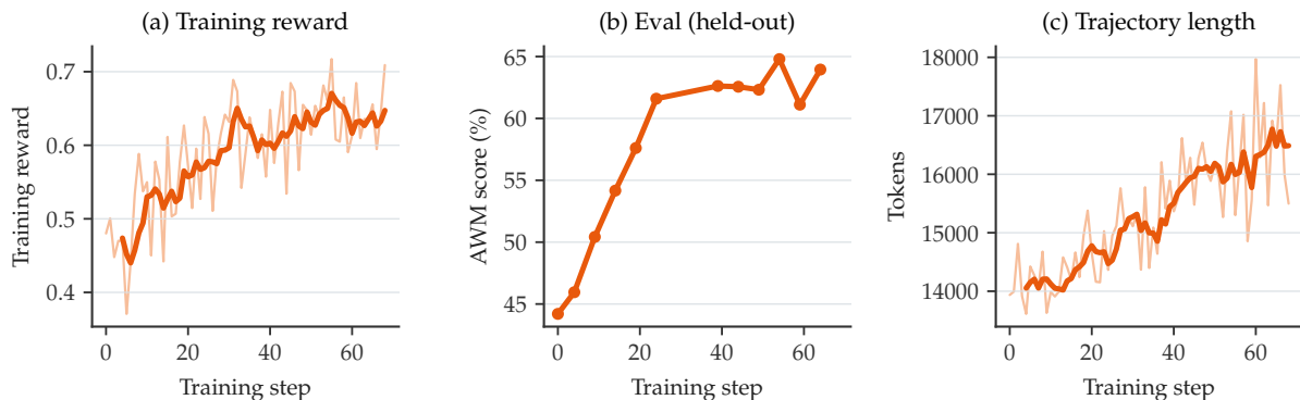
Figure 6: General Agent training dynamics , shown up to step 68, the checkpoint the pipeline carries forward. (a) Training reward; (b) held-out AWM score, scored by the in-loop training-time harness; (c) trajectory length in tokens. Light curves are per-step values and dark curves a 5-step moving average.
