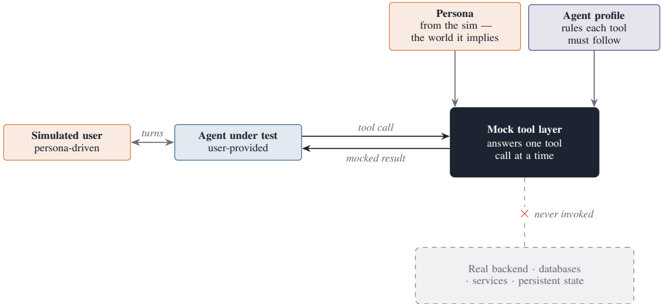
Figure 8. Tool-boundary mocking. As the simulated user and the agent under test exchange turns, each tool call the agent makes is answered by a mock tool layer parameterised by the persona and the agent profile. Only the tool boundary is mocked.
