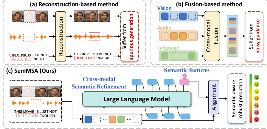
Figure 1: Framework comparison between (a) reconstruction-based methods, (b) fusion-based methods, and (c) our SemMSA. Compared with existing methods, SemMSA refines and fully integrates sentiment-relevant semantic information with the LLM to compensate for incomplete data.
