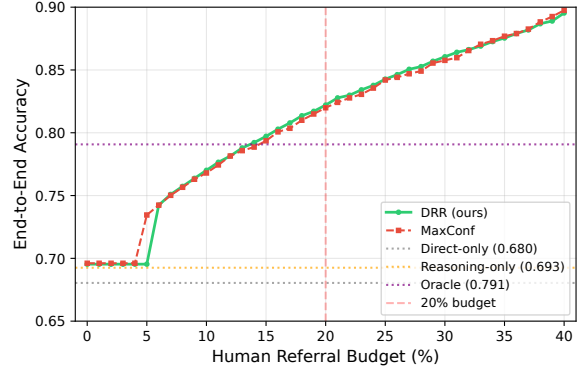
Figure 2: Accuracy-human budget trade-off. The x-axis varies the allowed human-referral budget, and the dashed line marks the operating point used in Table 1. Dotted horizontal lines show automated reference points. The curves show how different escalation policies convert limited human review into end-to-end accuracy during cold-start rollout.
