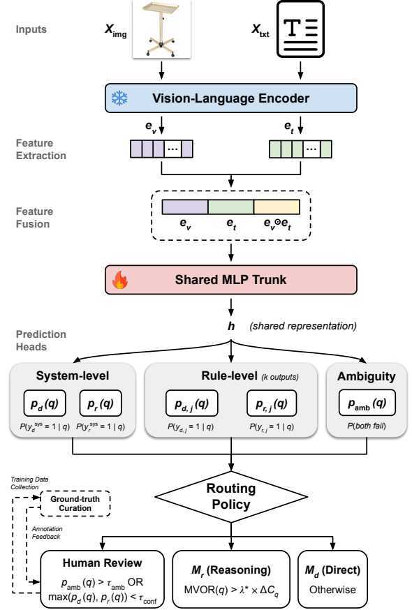
Figure 1: Overall DRR architecture for cost-aware three-way routing with human-feedback support.
